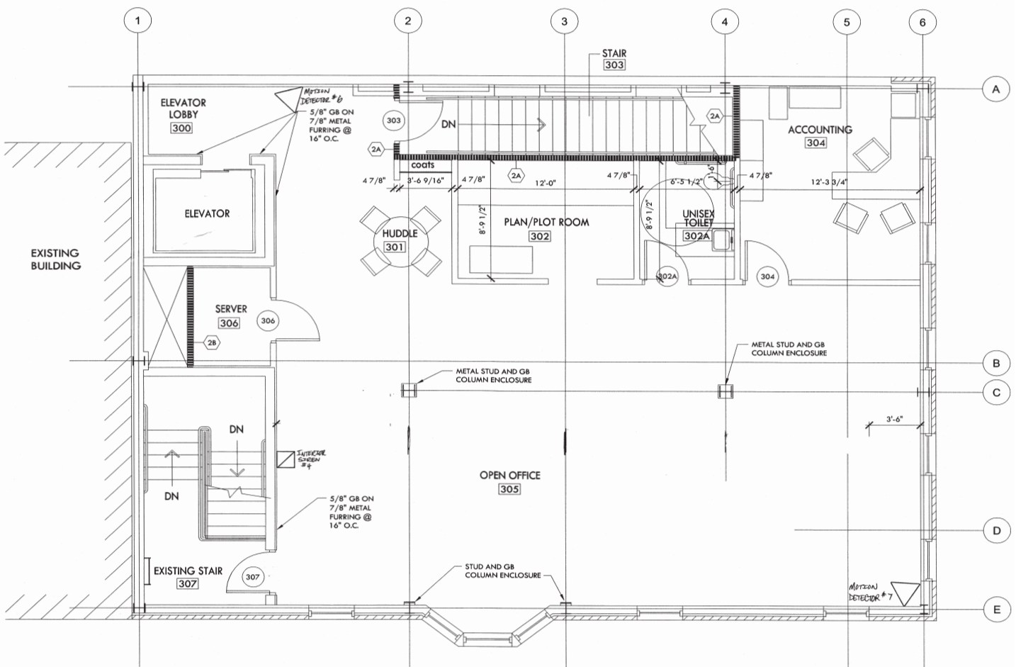
Third Floor Plan - 2,200 SF
