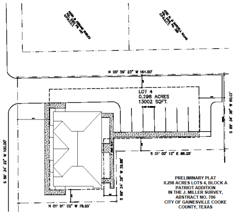
Site Plan - LOT 4 SCALE: 1" = 20'-0"
