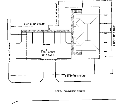
Site Plan - LOT 5 SCALE: 1" = 20'-0"
