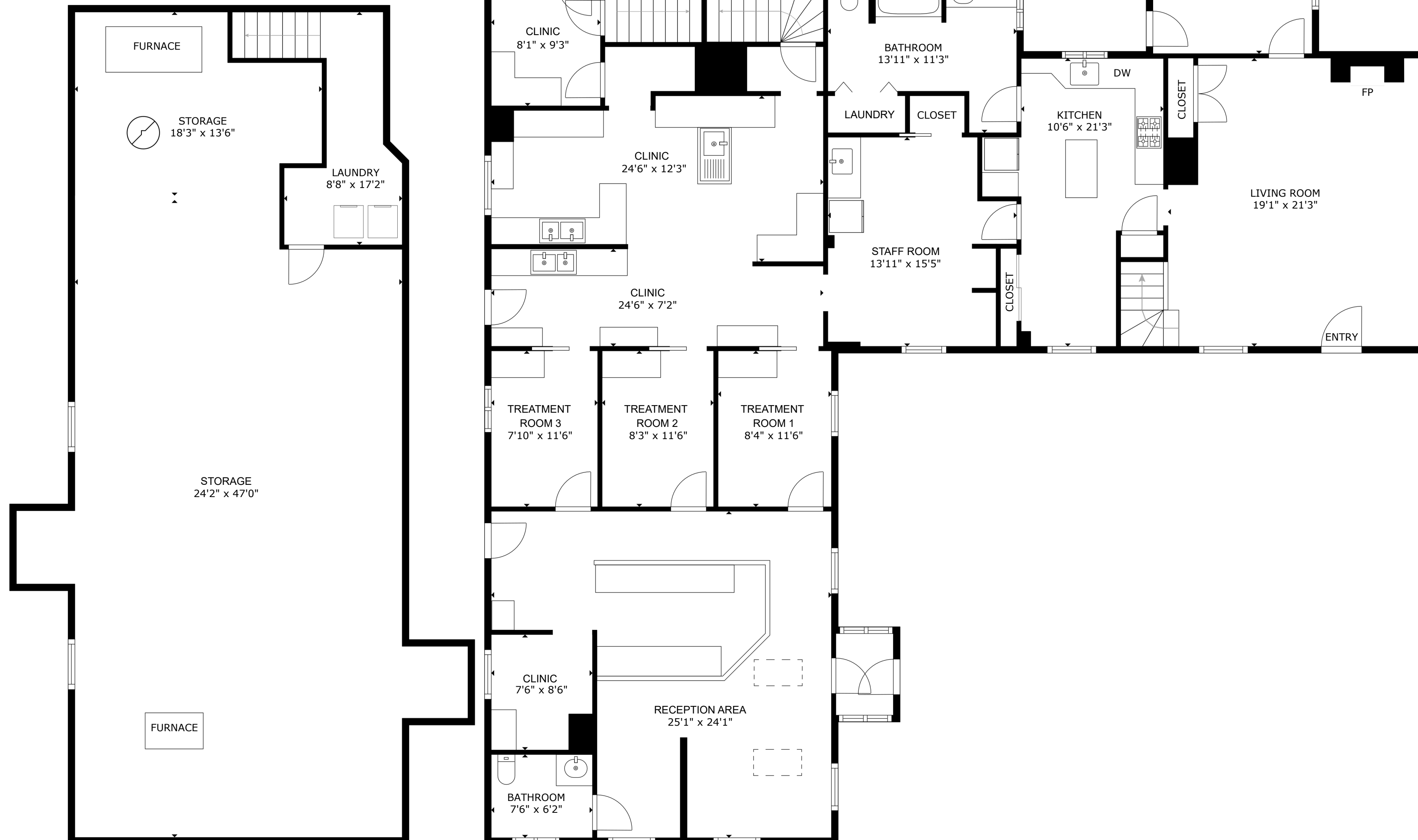
FLOOR 1
