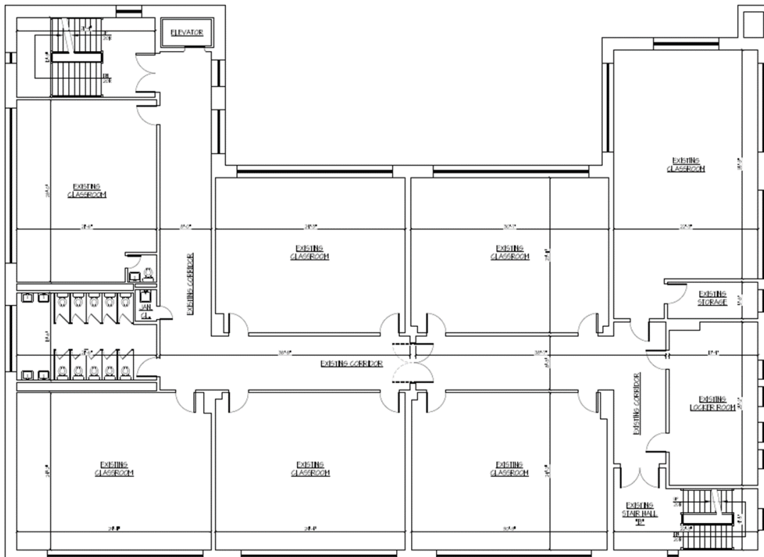
EXISTING 2nd FLOOR PLAN
