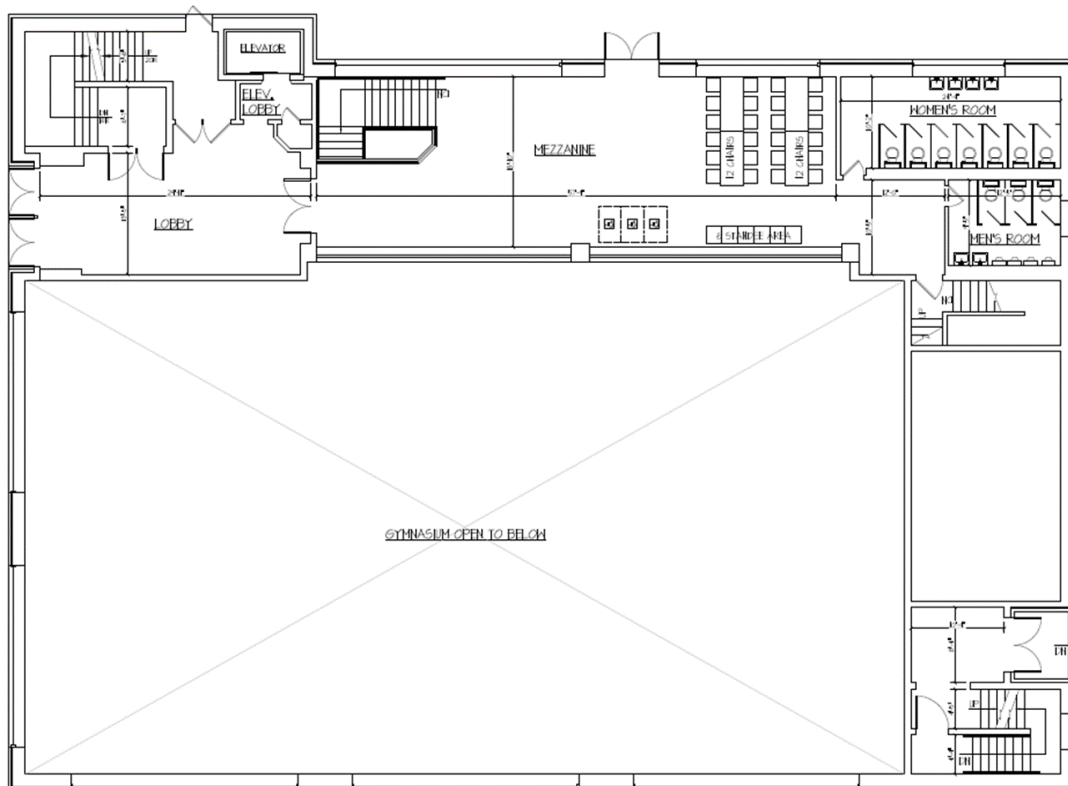
EXISTING MEZZANINE FLOOR PLAN
