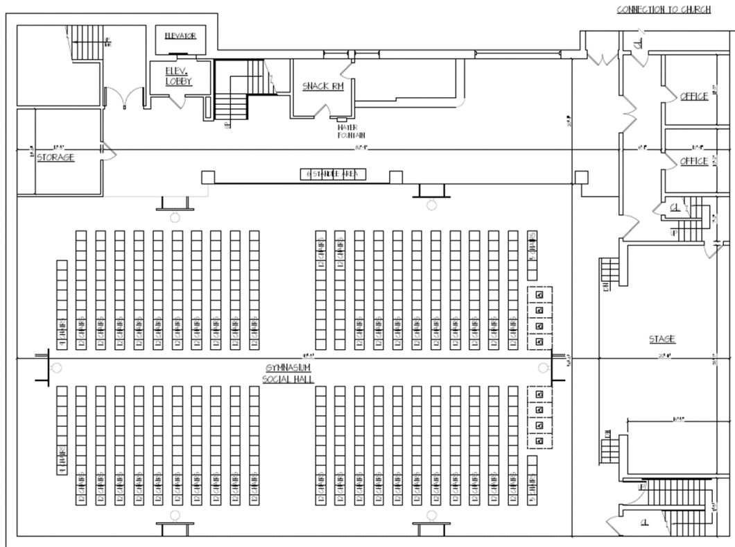
EXISTING CELLAR FLOOR PLAN
