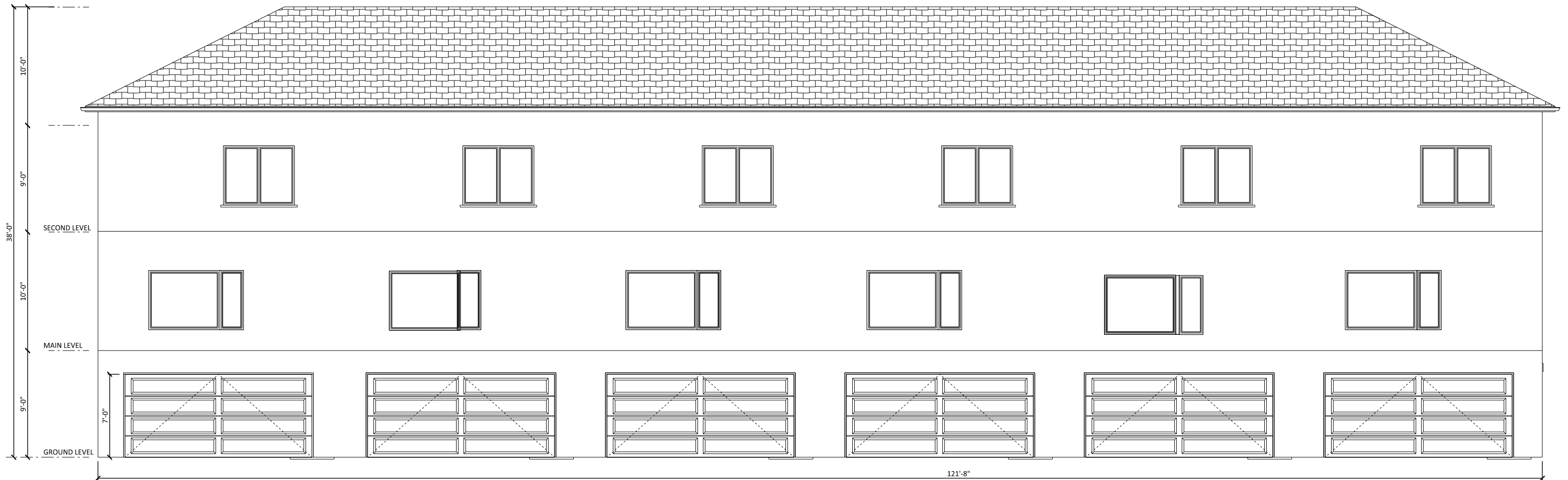
REAR ELEVATION
