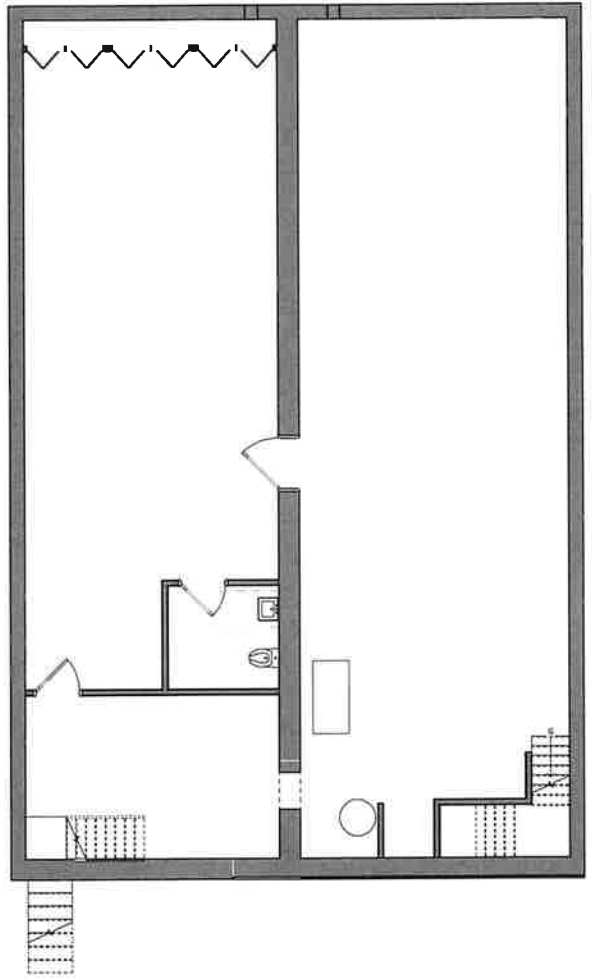
1 PLAN - LEVEL 00 - FLOOR PLAN - EXISTING 1/8" = 1'-0"
