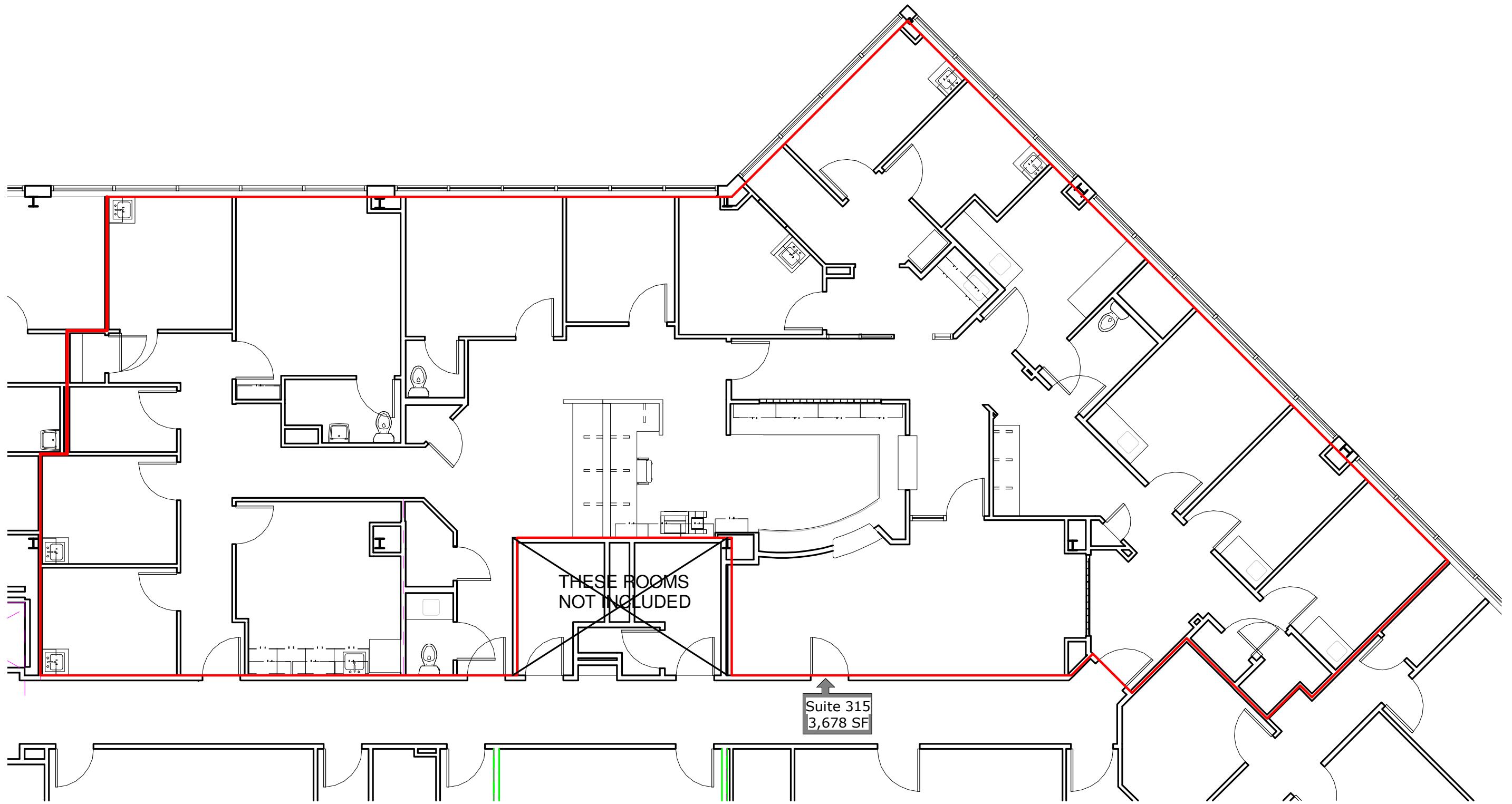
1 Level 3 Suite 315 New 1/8" = 1'-0"
