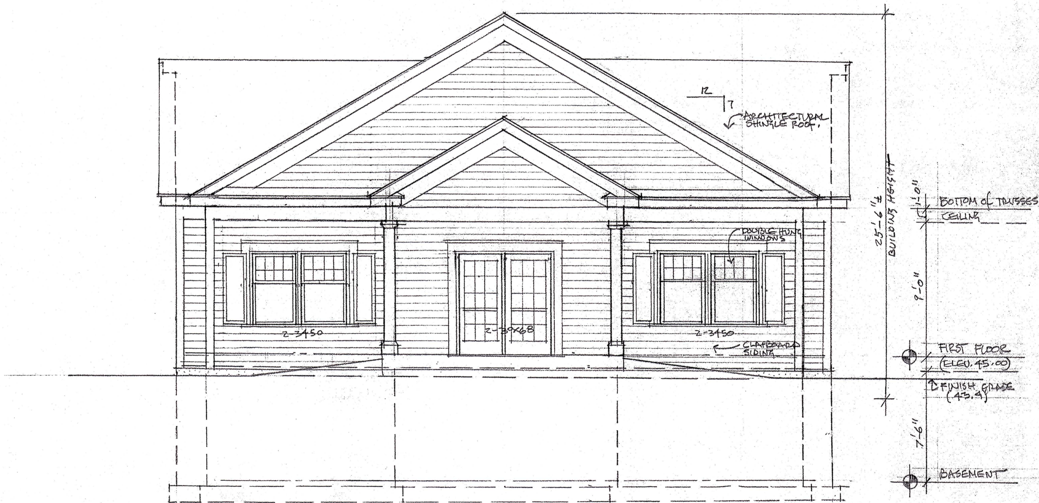
1 NORTH BUILDING ELEVATION AZ SCALE = 1/4" = 1'-0"
