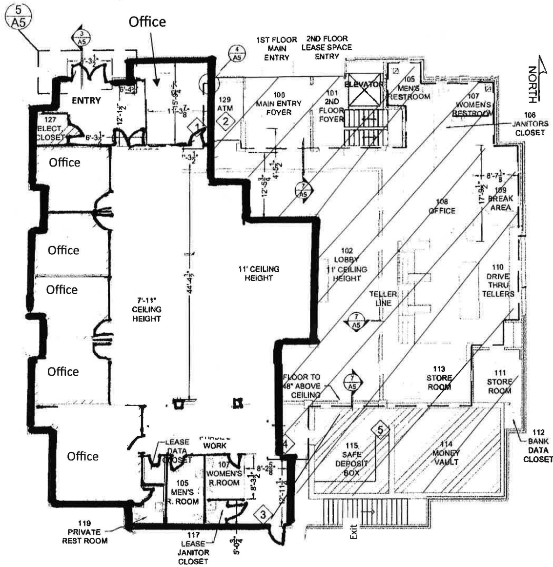
FLOOR PLAN 1/8" SCALE
