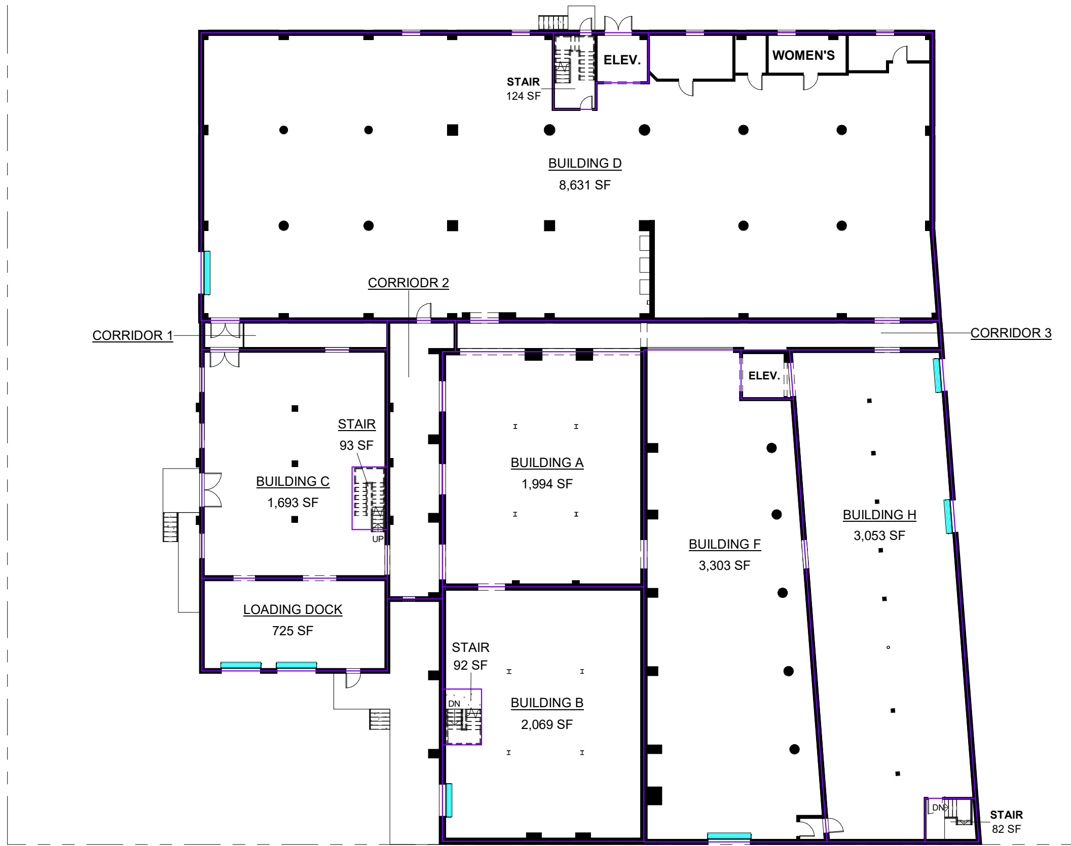
① FIRST FLOOR PLAN 1" = 20'-0"
