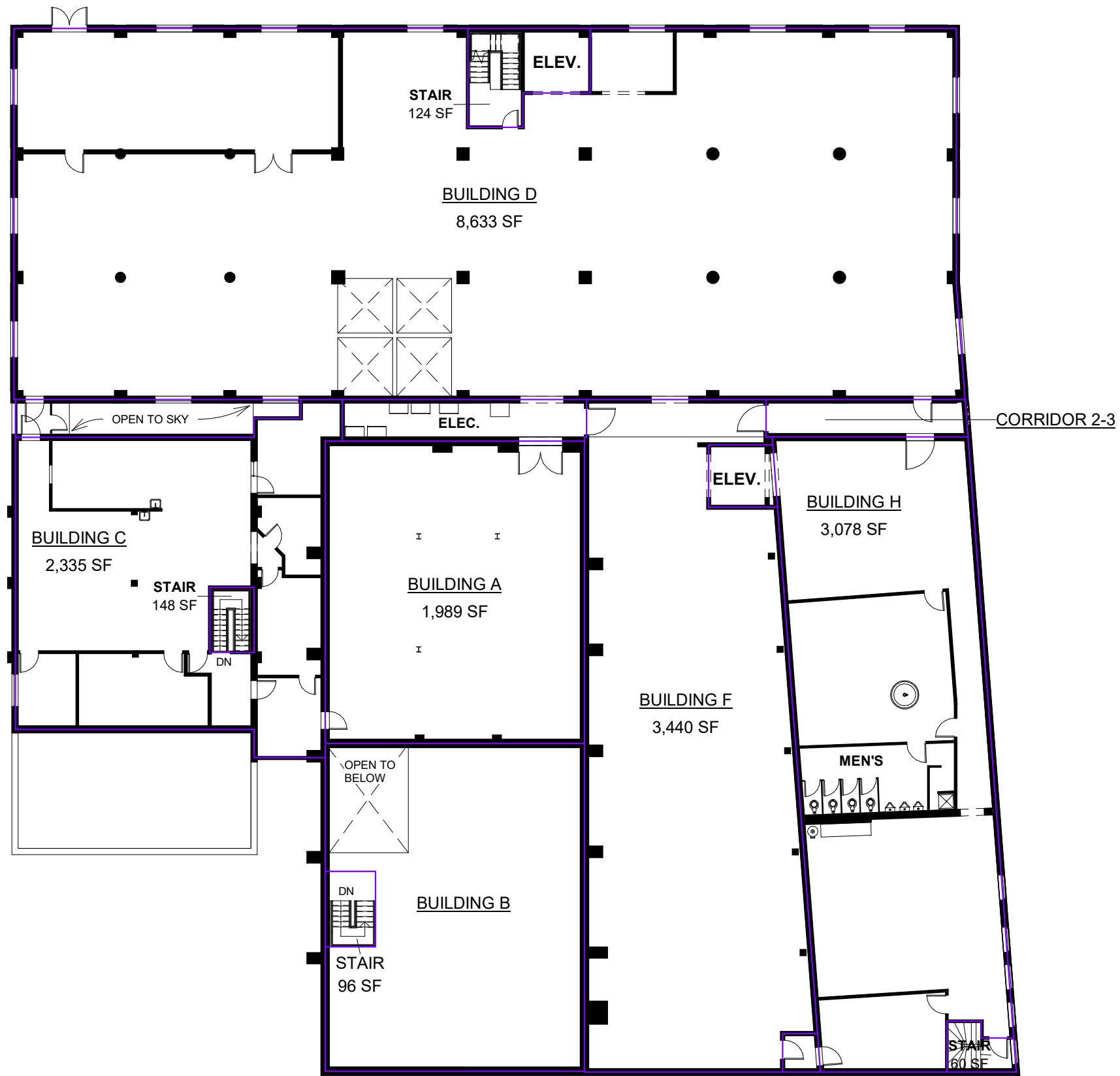
② SECOND FLOOR PLAN 1" = 20'-0"
