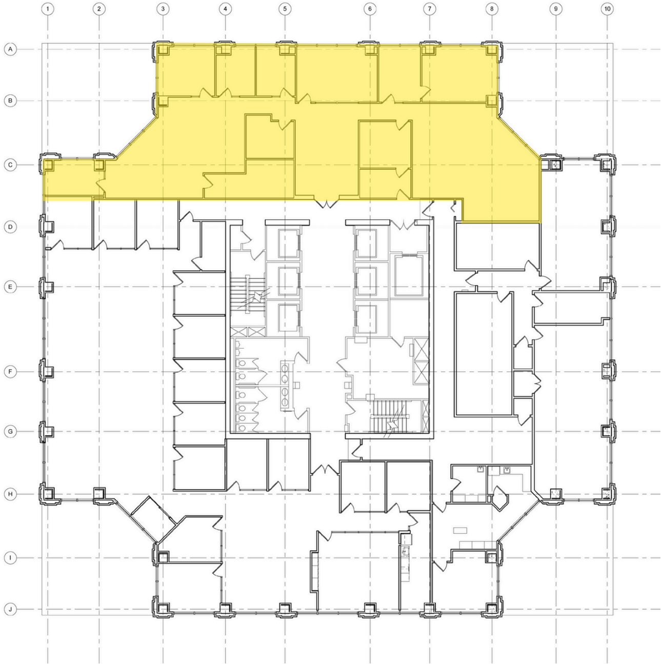
EIGHTH FLOOR PLAN - EASTERN SUITE - BOMA A-011 1/8" = 1'-0"
