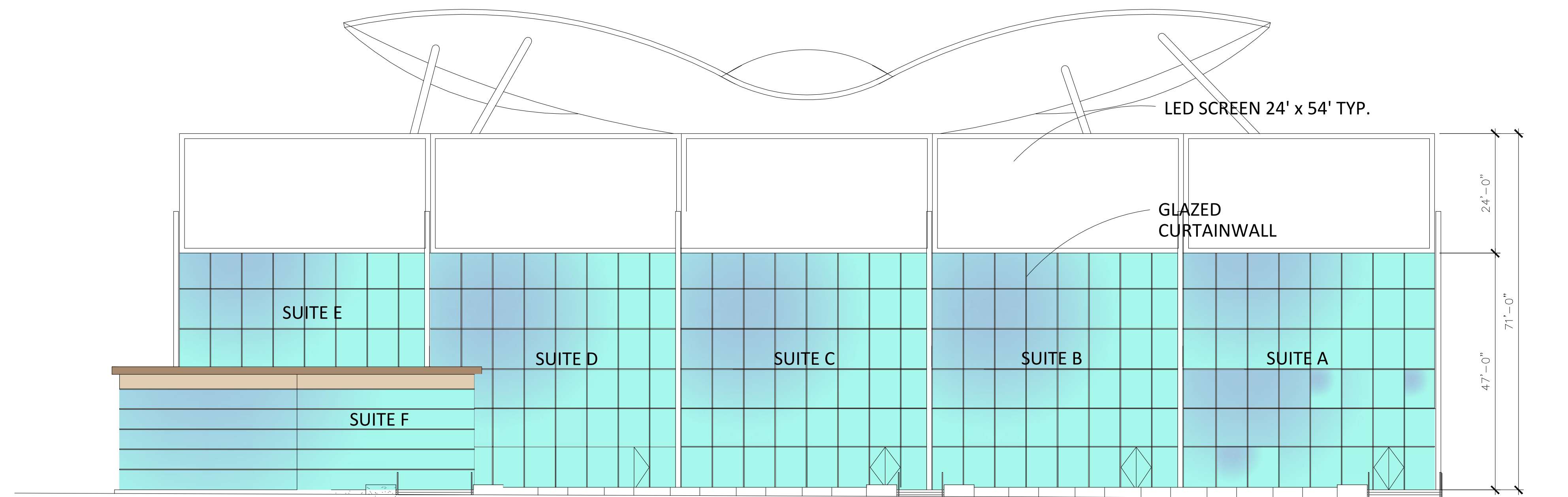
Front Elevation
