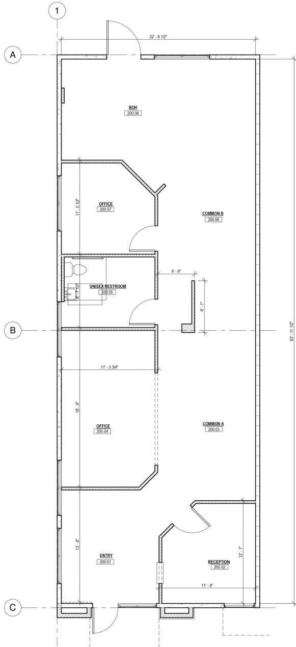
① EXISTING FIRST FLOOR PLAN 1/4" = 1'-0"
