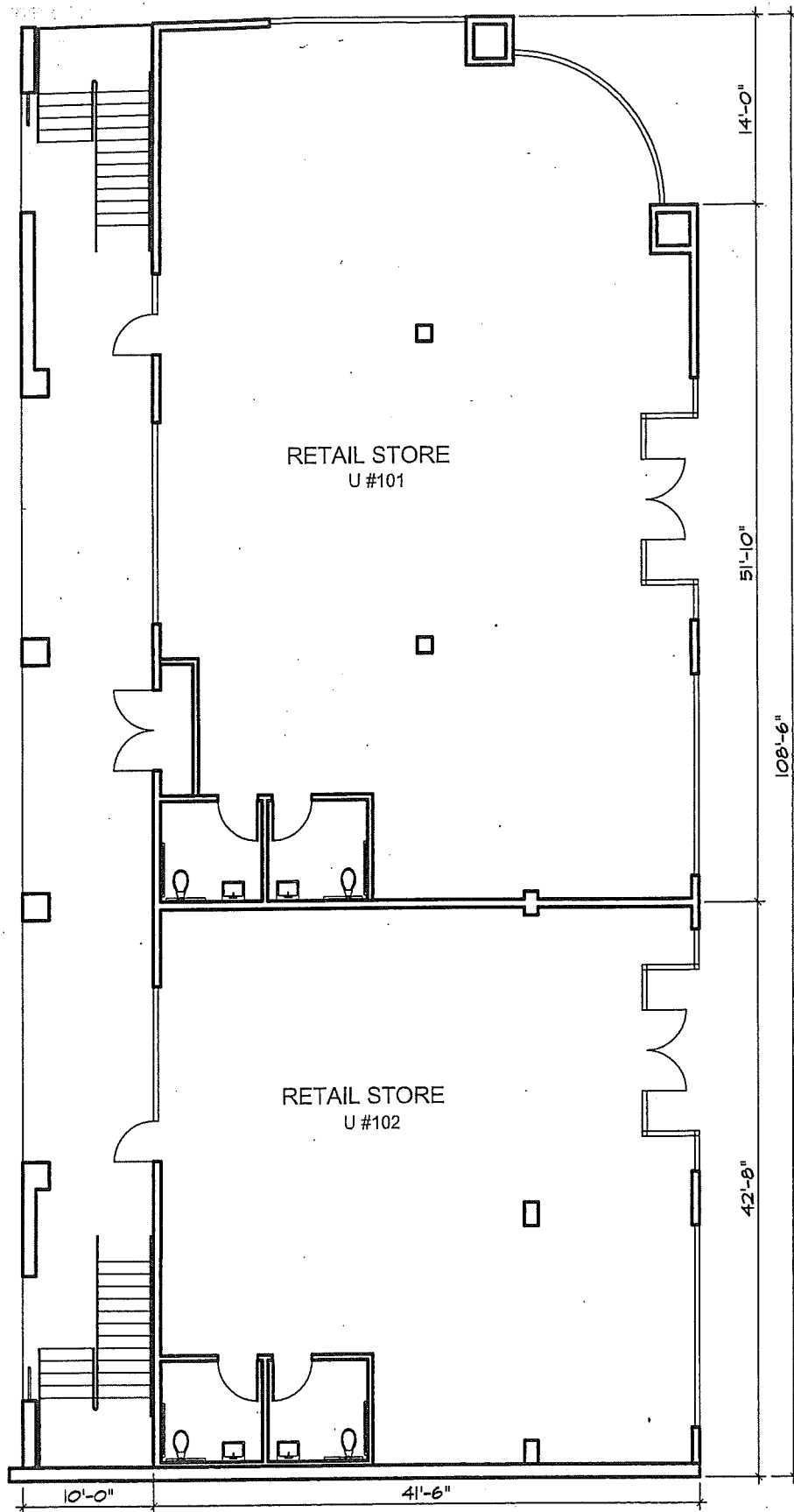
1ST. FLOOR PLAN 745 E. GARVEY AVE.
