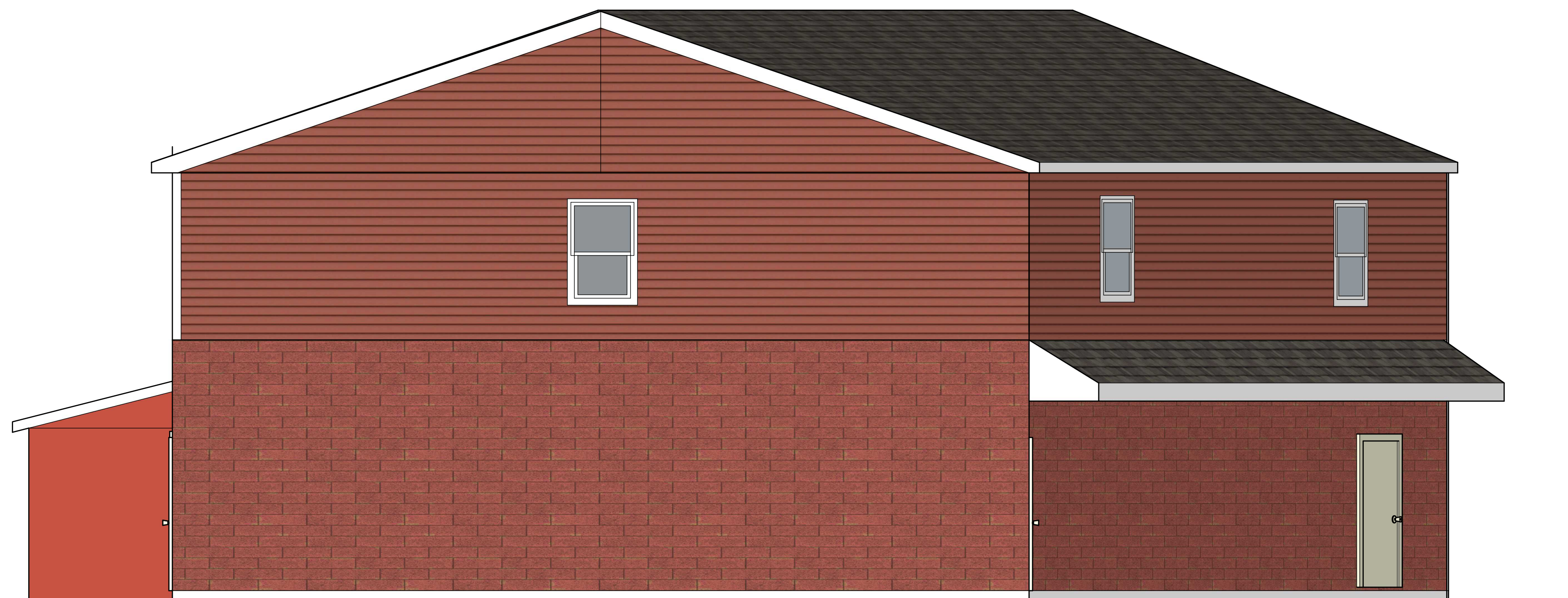
West Elevation
