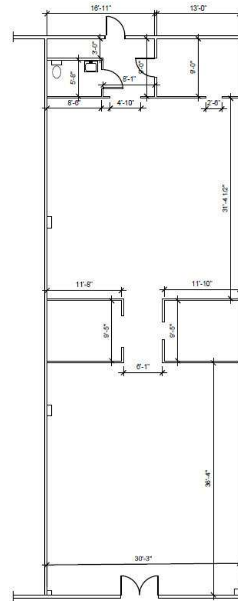
2013 - FLOOR PLAN SCALE: 1/8"=1'-0"
