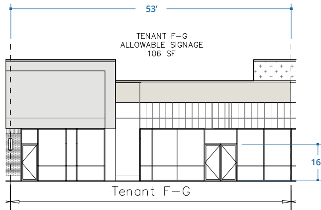
Ⓜ ELEVATION 1" = 10'
