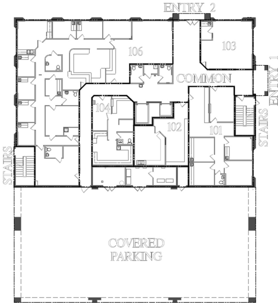
FLOOR PLAN (GROUND LEVEL) SCALE: 1/8" = 1'-0"
