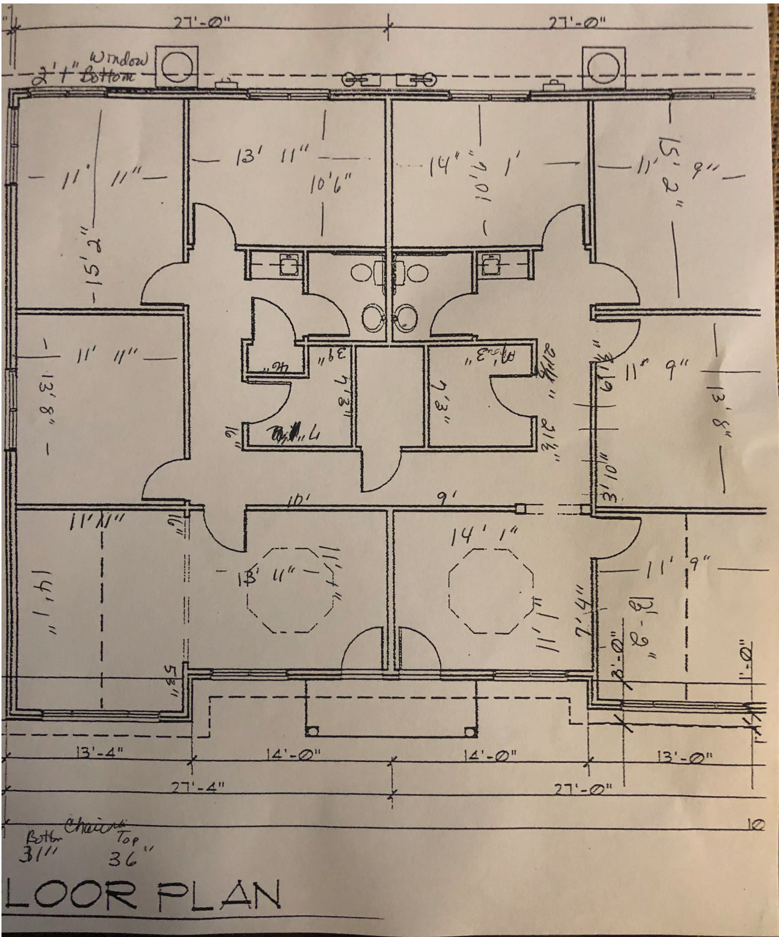
Floor Plan - 1901 Macy Drive, Roswell, GA 30075
