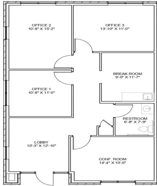
01 TYPICAL FLOOR PLAN - 1,187 SF SCALE: 1/8" = 1'-0"
