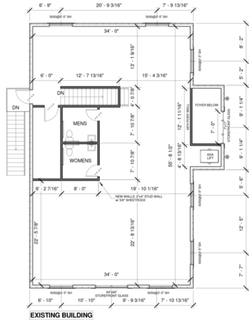
① Level 2 2,085 SF 1/8" = 1'-0"
