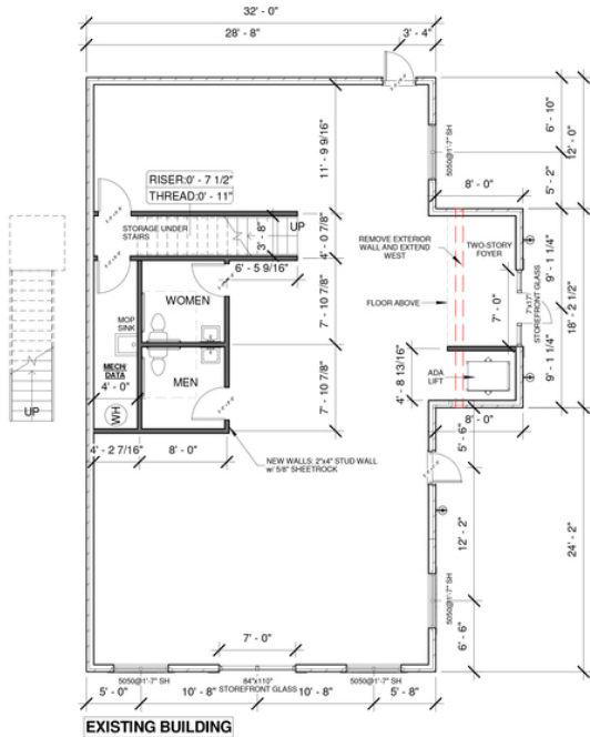
① Level 1 1,886 SF 1/8" = 1'-0"
