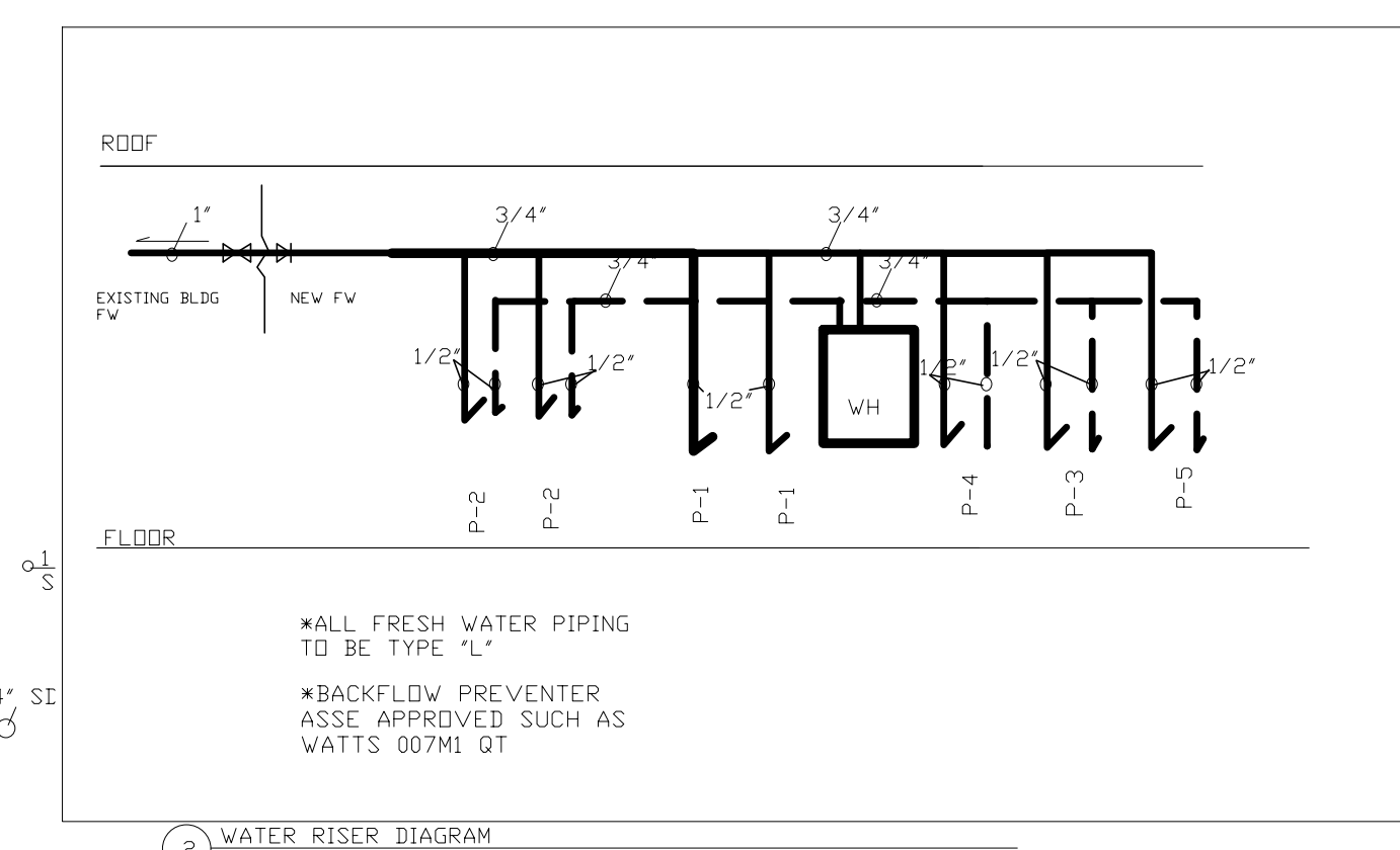
2. WATER RISER DIAGRAM NO SCALE
