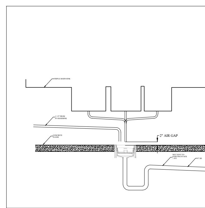
4. TRIPLE SINK / FLOOR SINK DRAIN DETAIL NO SCALE
