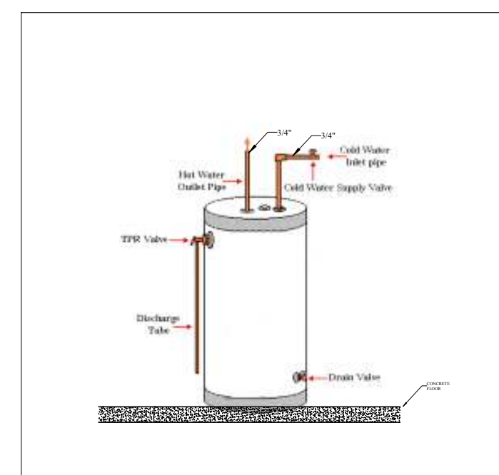
3. WATER HEATER DETAIL NO SCALE
