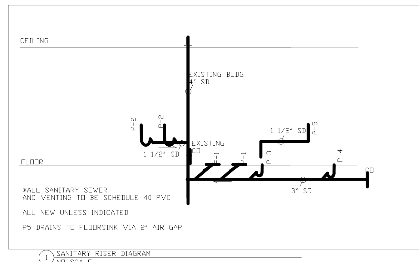
1. SANITARY RISER DIAGRAM NO SCALE
