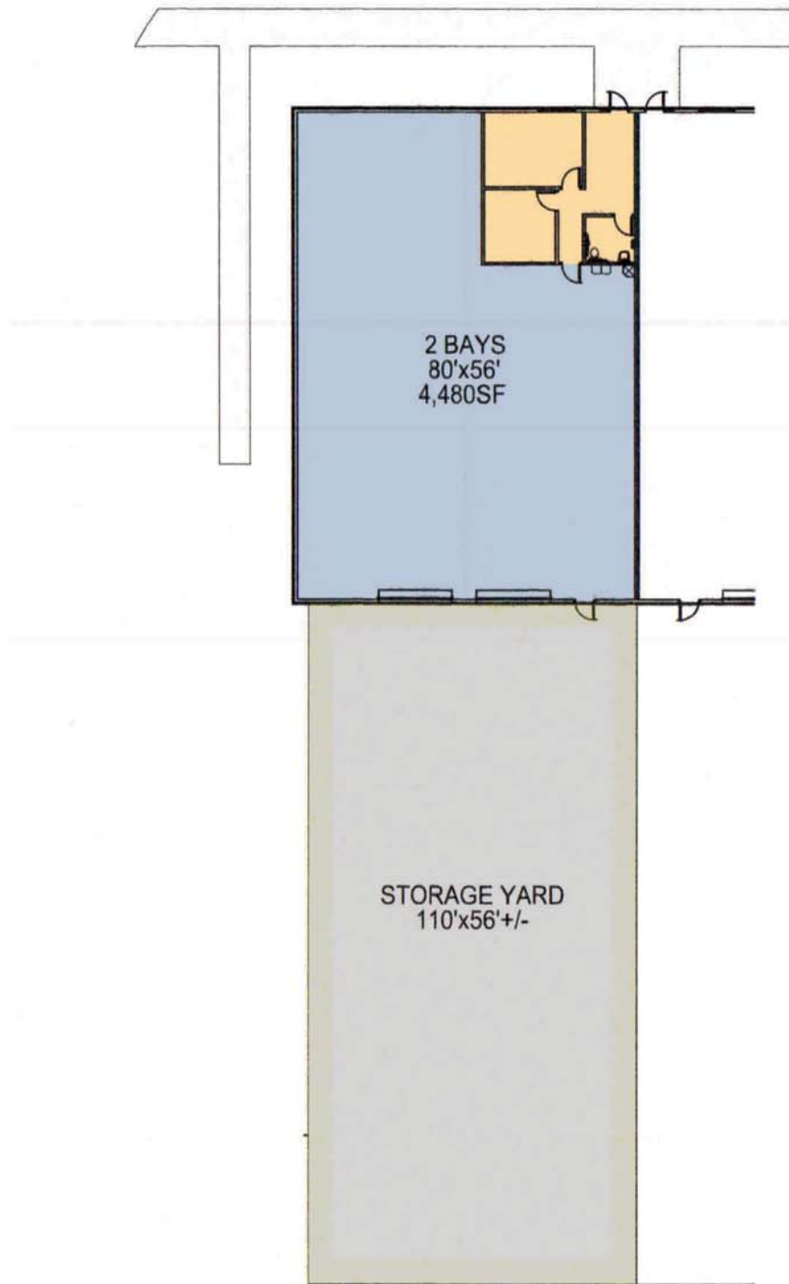
2 BAY PLAN
