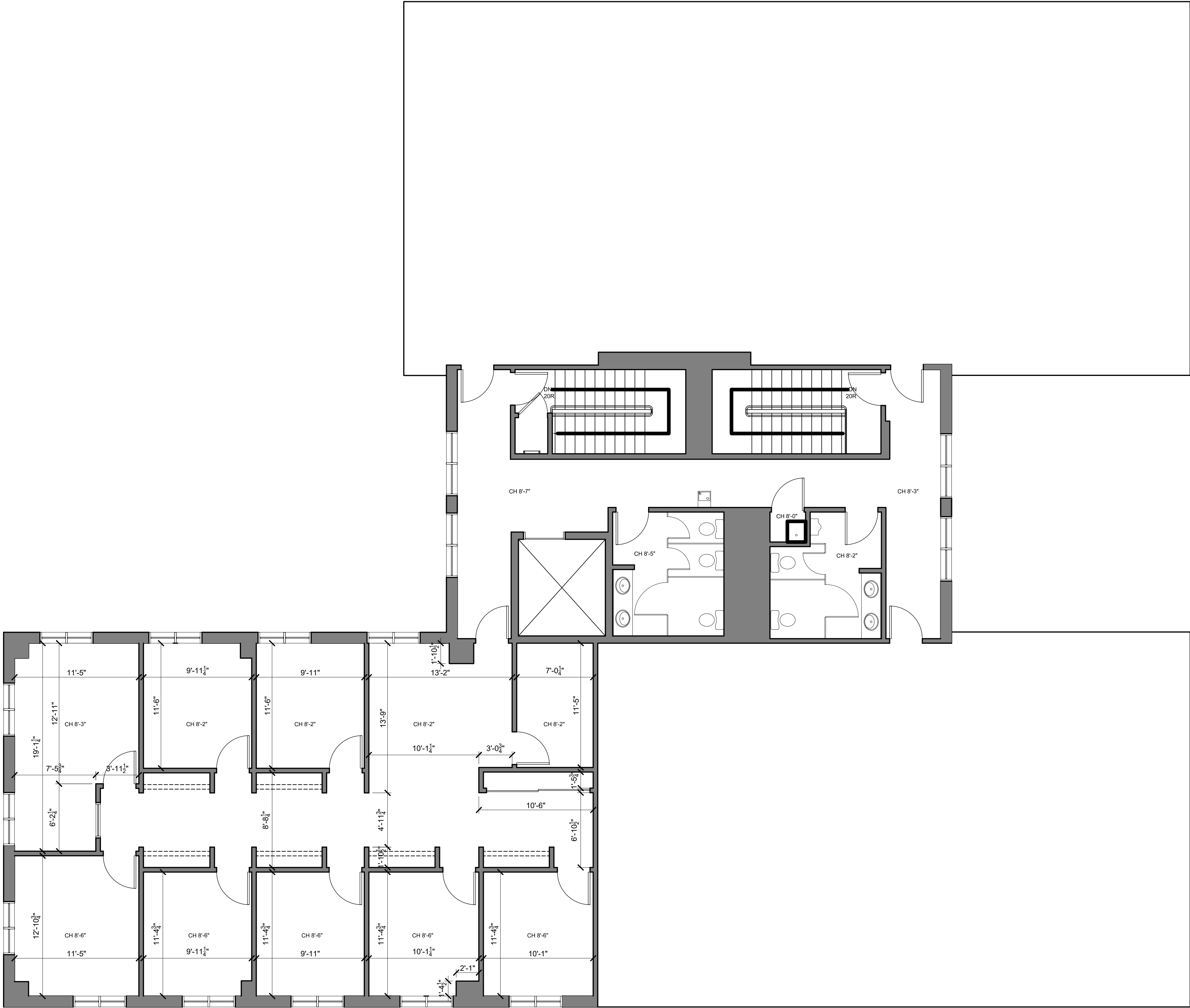
1 THIRD FLOOR PLAN 1/8" = 1' - 0"
