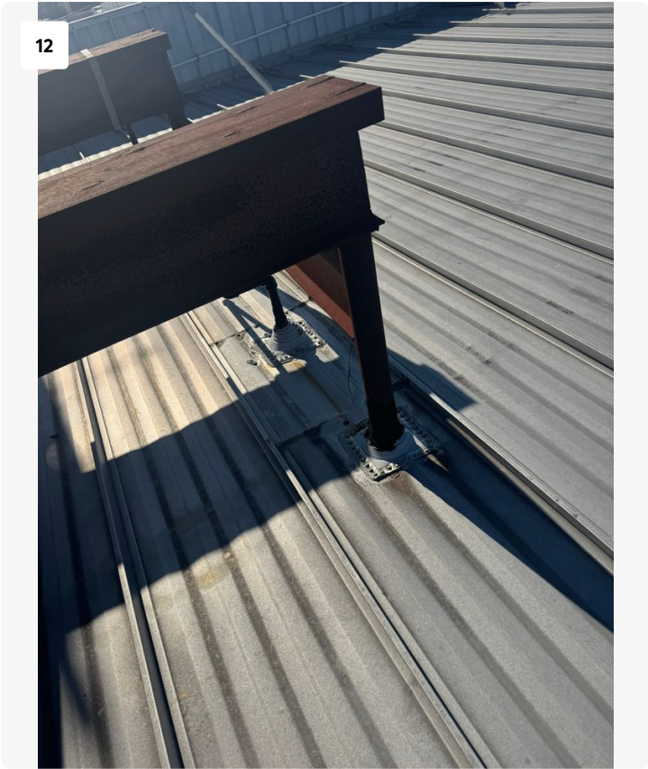
Iron supports have appropriate boot flashings at base
