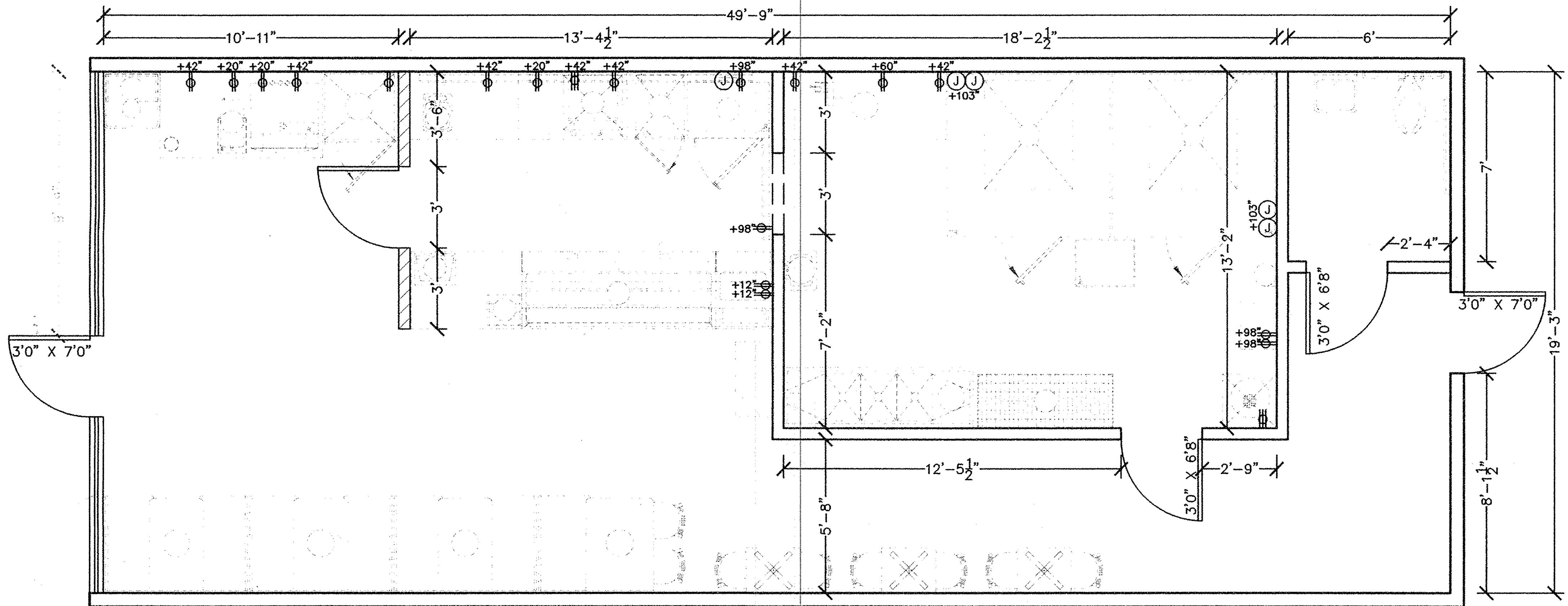
3 ELECTRIC AND DIMENSION PLAN SCALE: 1/4" = 1'
