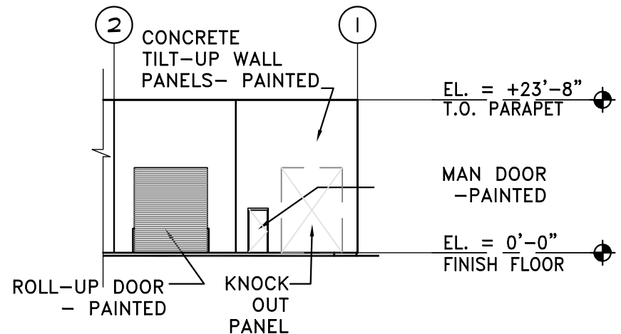
PARTIAL REAR ELEVATION
