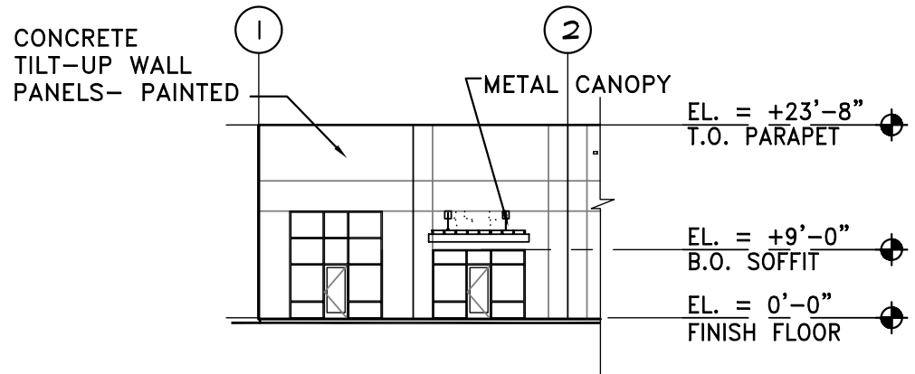
PARTIAL FRONT ELEVATION
