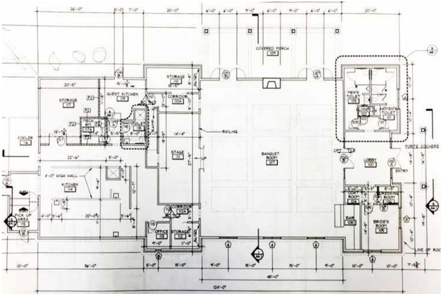
1 FLOOR PLAN A1.1 1/8" = 1'-0"
