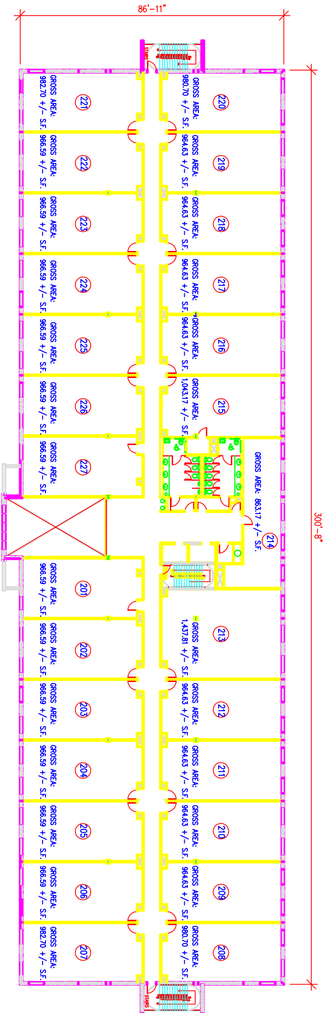
OFFICE BUILDING SECOND FLOOR PLAN
