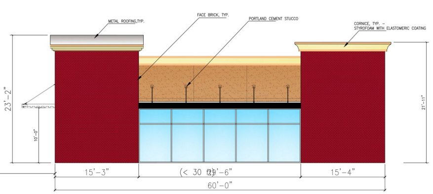
3 BLDG-2 NORTH ELEVATION 3/16" = 1'-0" (NOTE: 15% OF WALL AREA UP TO 10FT (600 S.F.) AFF = 90 S.F.)
