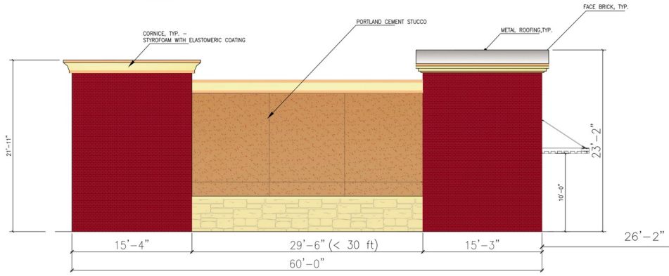
2 BLDG-2 SOUTH ELEVATION 3/16" = 1'-0"
