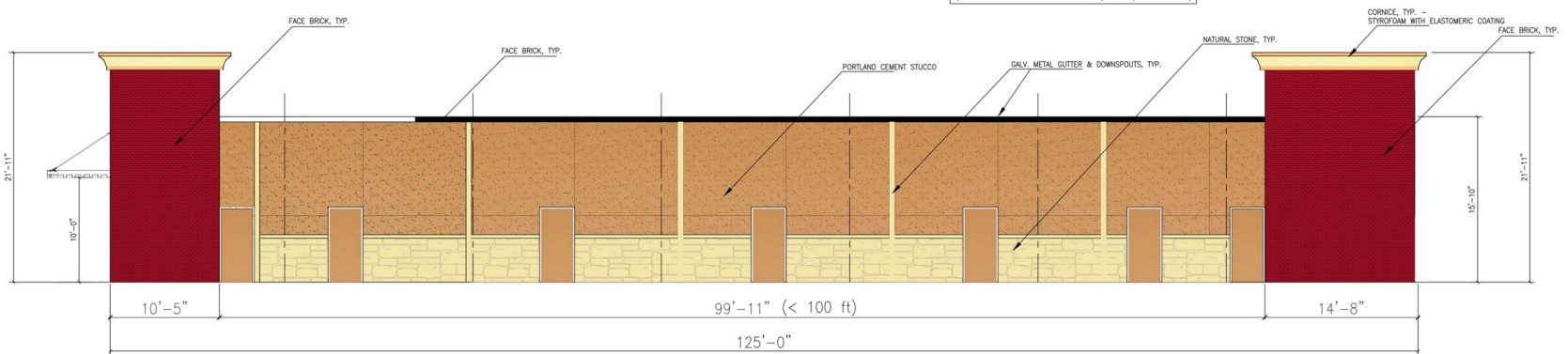
4 BLDG-2 WEST ELEVATION 3/16" = 1'-0"
