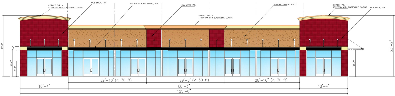
1 BLDG-2 EAST ELEVATION 3/16" = 1'-0"
