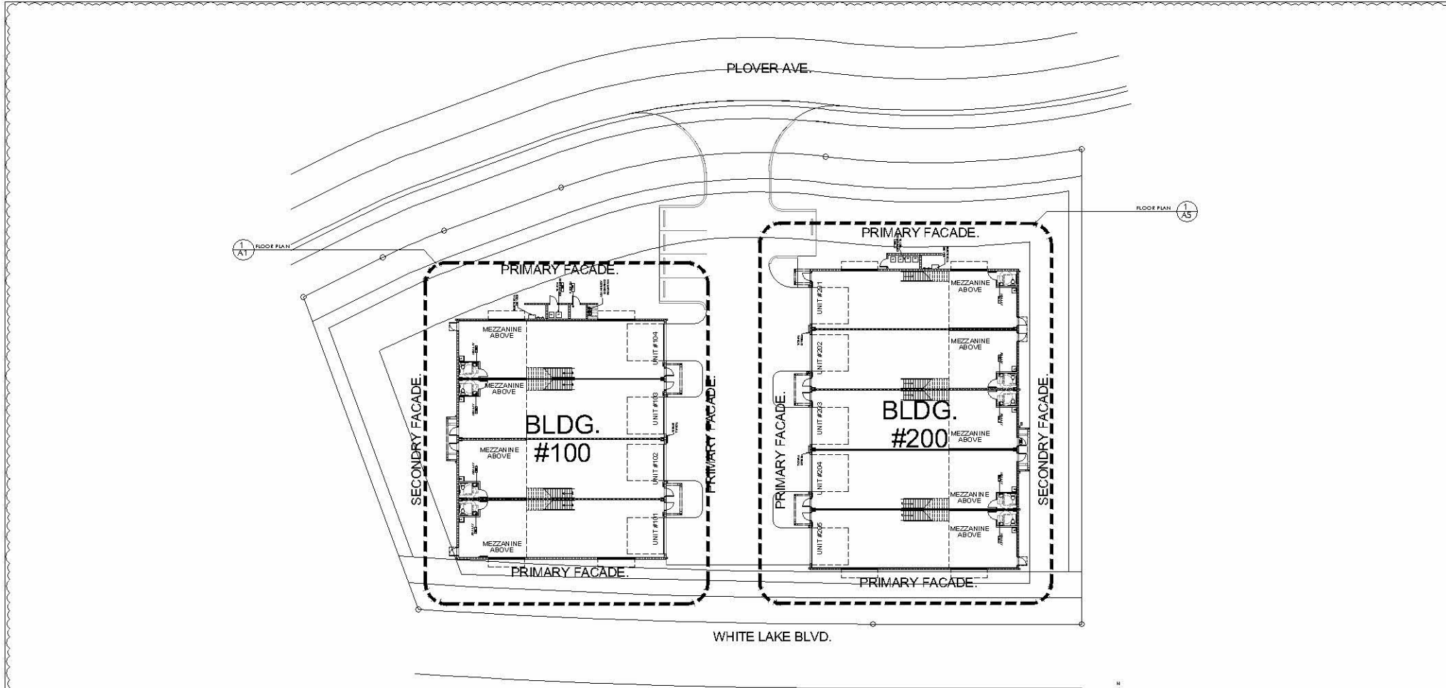
1 A-0 PROPOSED KEY PLAN SCALE: 1/8"=1'-0"
