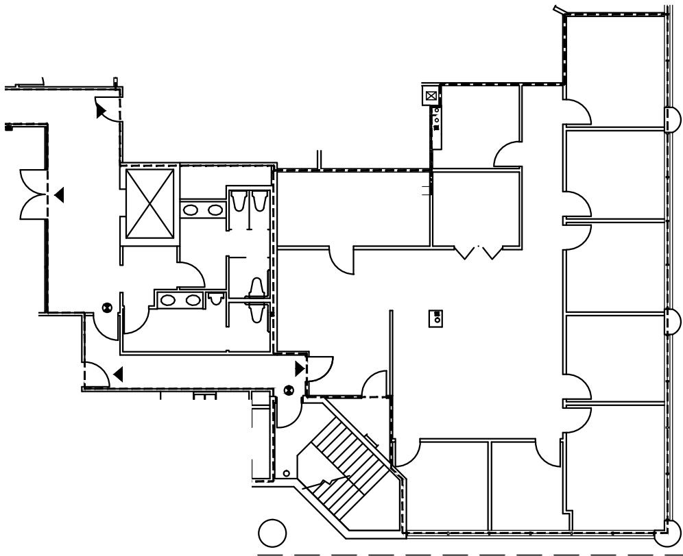
① FOURTH FLOOR PLAN—SUITE 403 SCALE_1"=16'-0"
