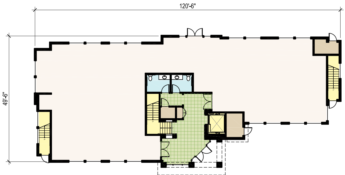
BUILDING 2 - GROUND FLOOR PLAN
