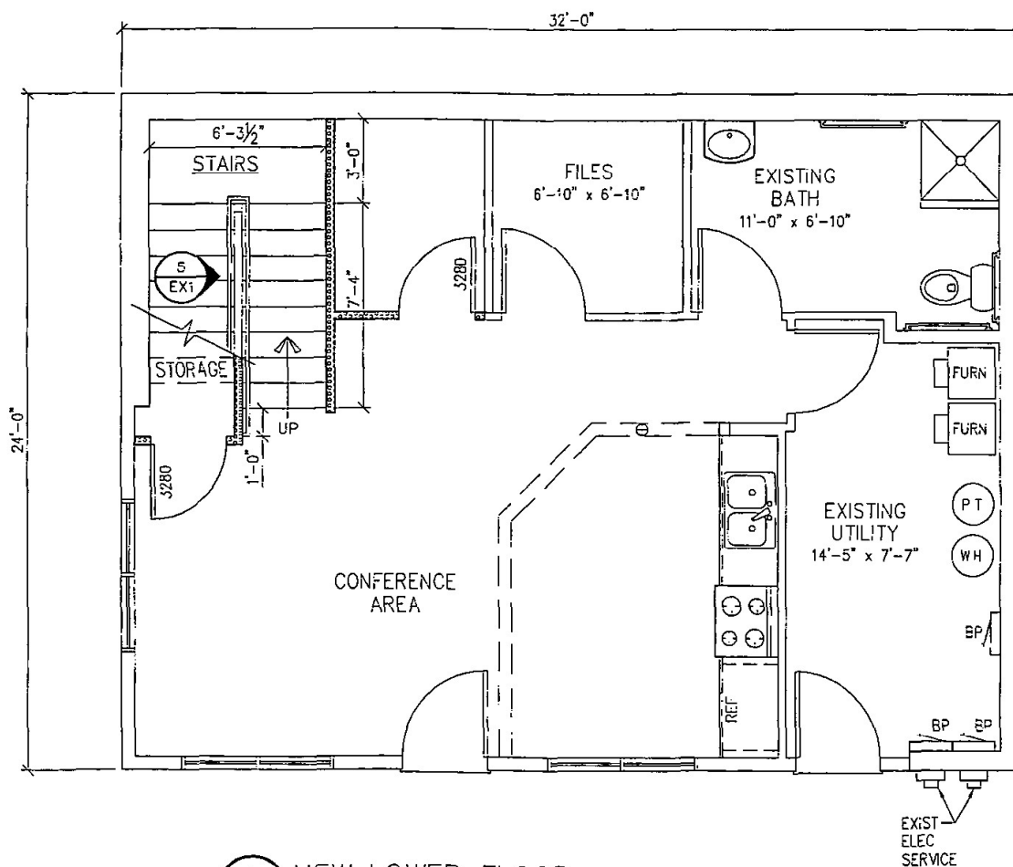
3 NEW LOWER FLOOR EX1 SCALE 1/4" = 1'-0"
