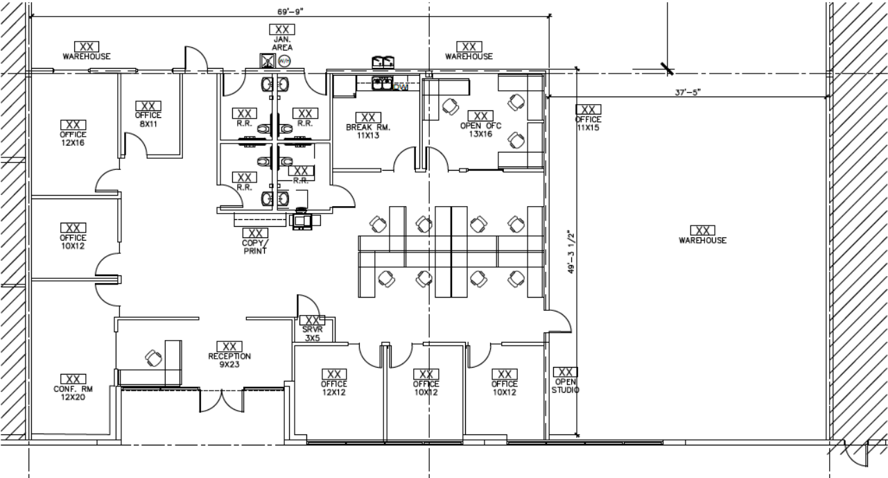
1 PRELIM. FLOOR PLAN SCALE: 1/16"=1'-0" OFFICE SF: 3,315 SF
