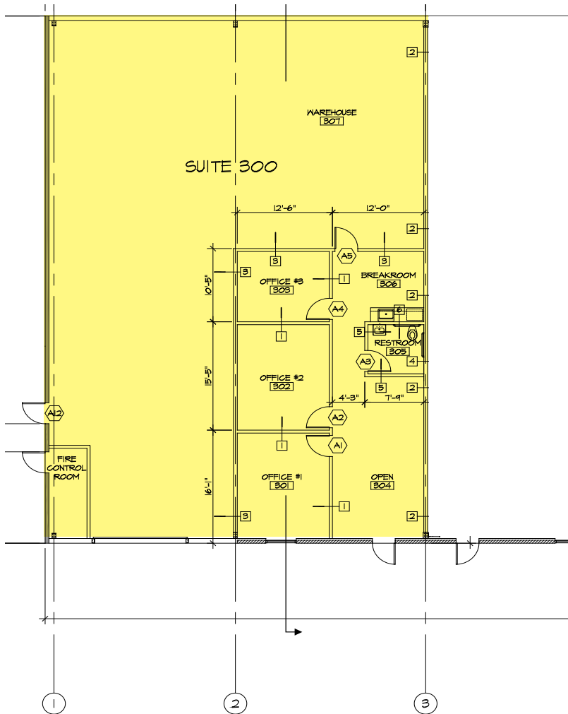
A FLOOR PLAN WITH OFFICE LAYOUT A.2.1 PLAN SCALE: 1/8" = 1'-0"
