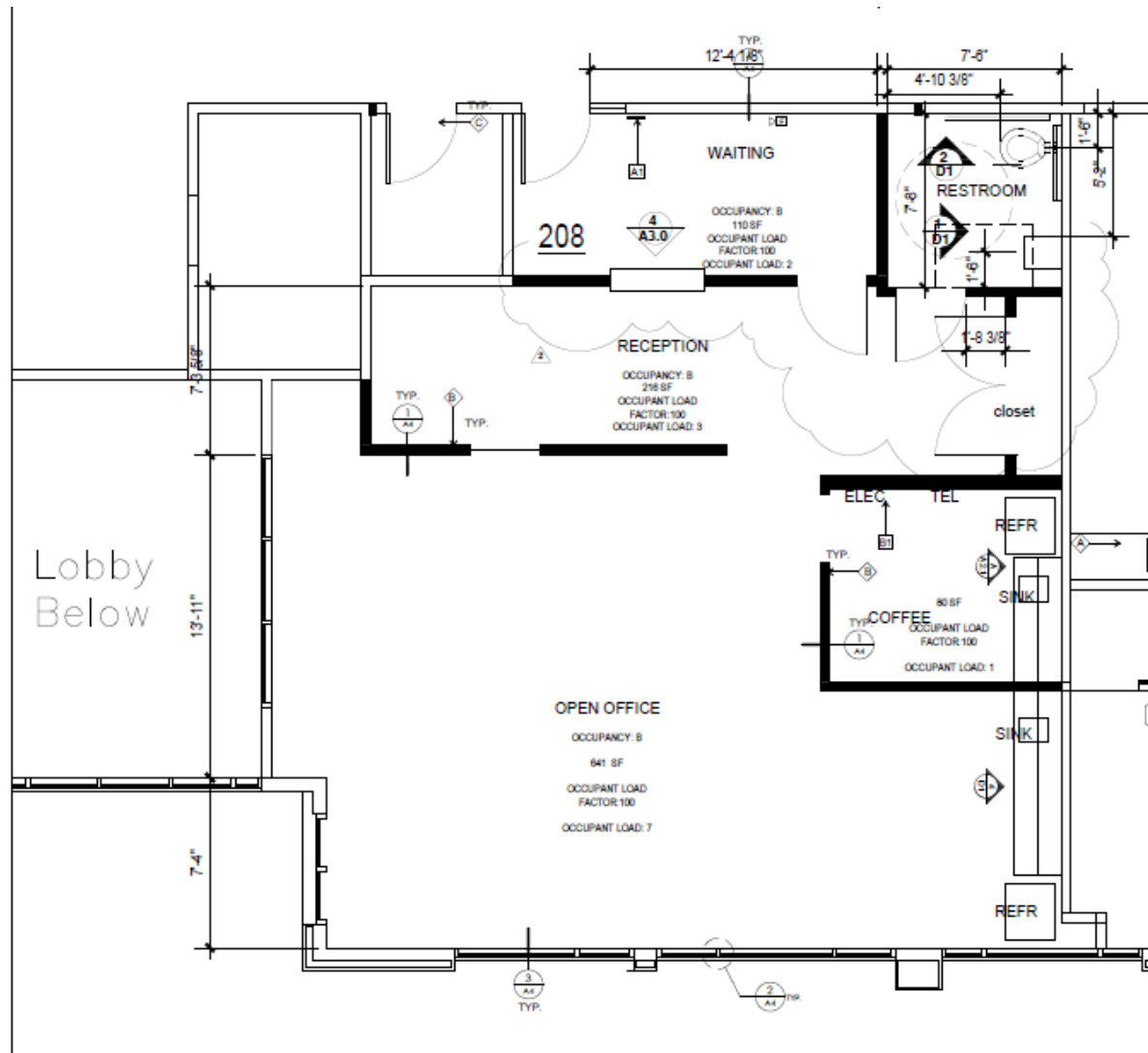
FLOOR PLAN 3/8" = 1'-0"
