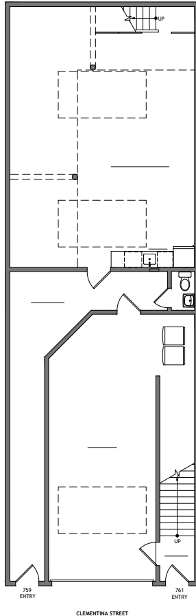
CLEMENTINA STREET GROUND FLOOR PLAN
