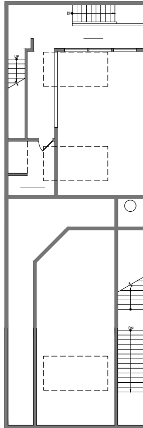
CLEMENTINA STREET MEZZANINE LEVEL PLAN
