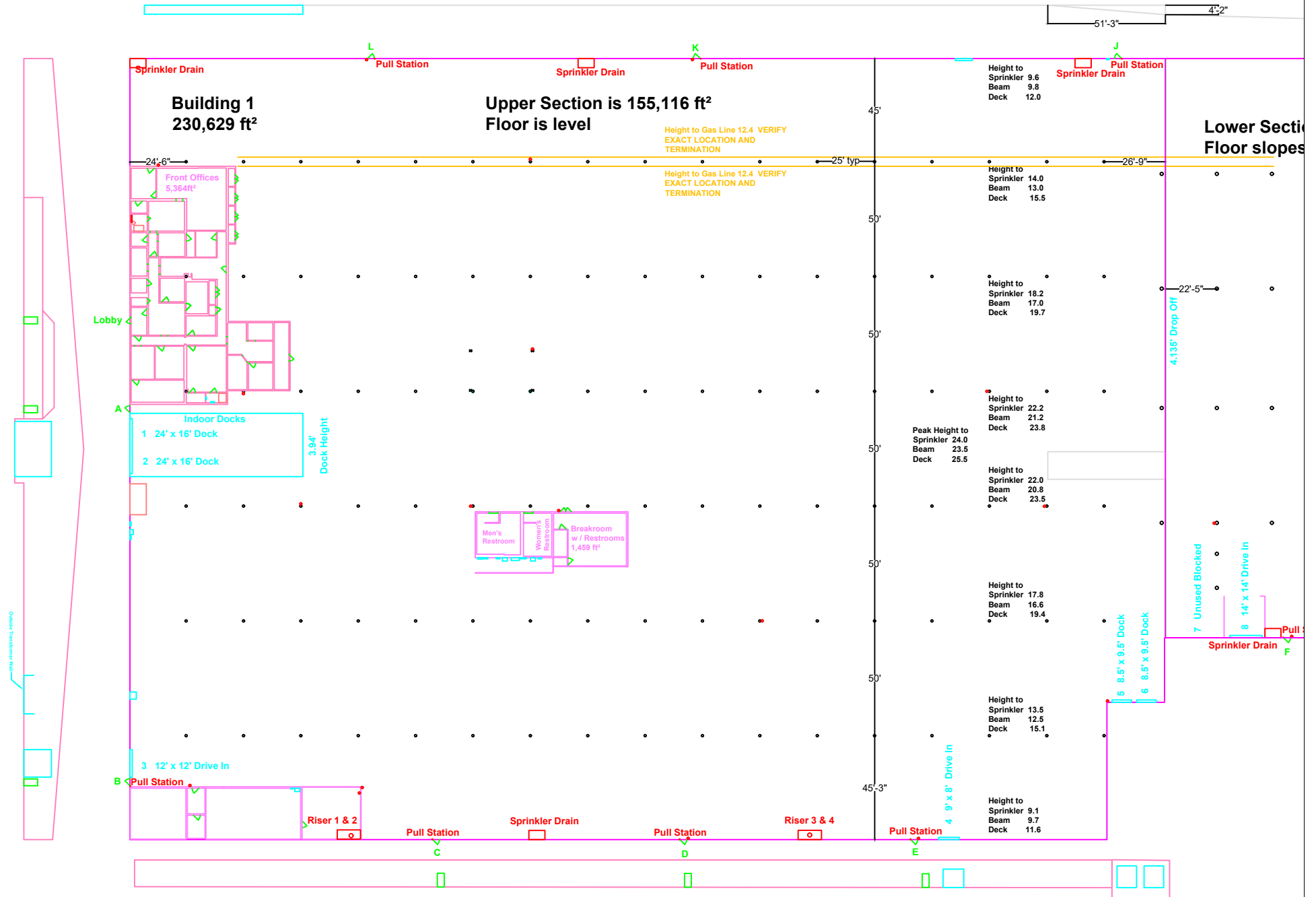
Floors and Dock Section
