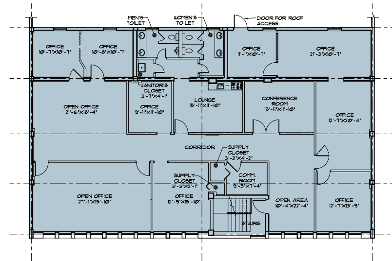
±3,554 SF 2 nd Floor Office
