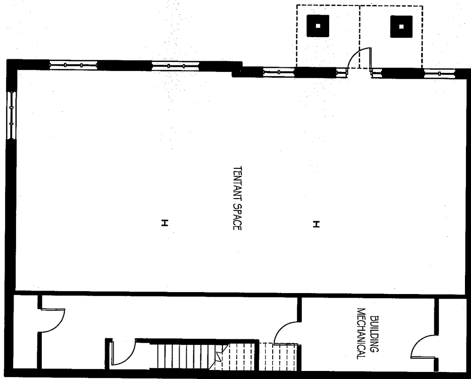
LOWER LEVEL FLOOR PLAN 1/8" = 1'-0"
