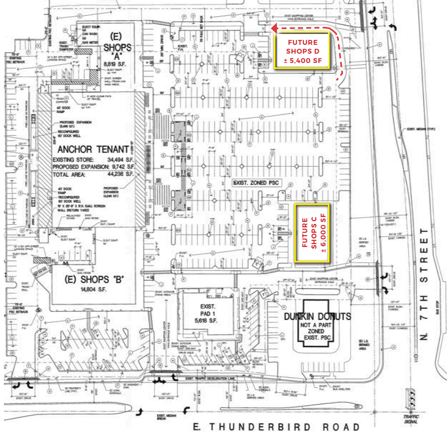
PROPOSED SITE PLAN (OPTION B)
