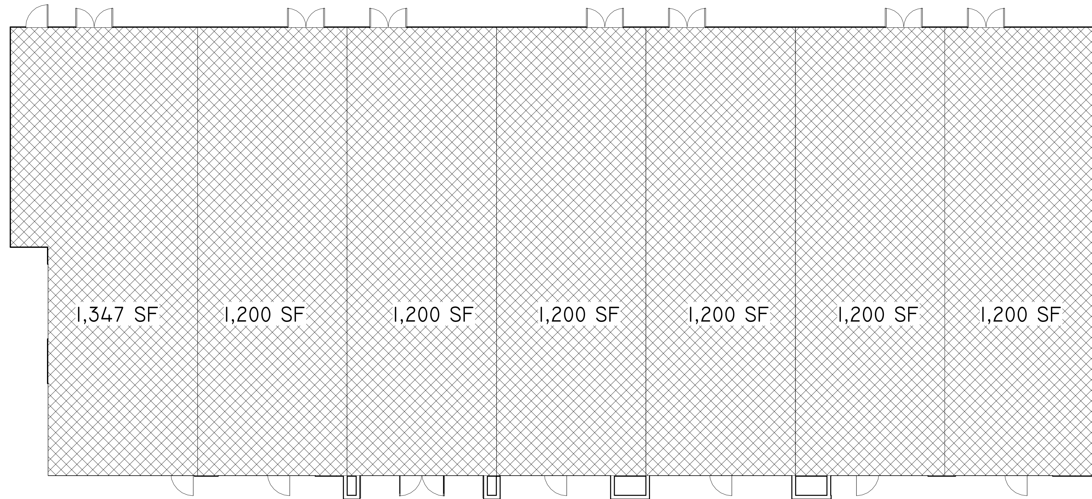
① FLOOR PLAN - BLDG A TENANT SF 1/8" = 1'-0"
