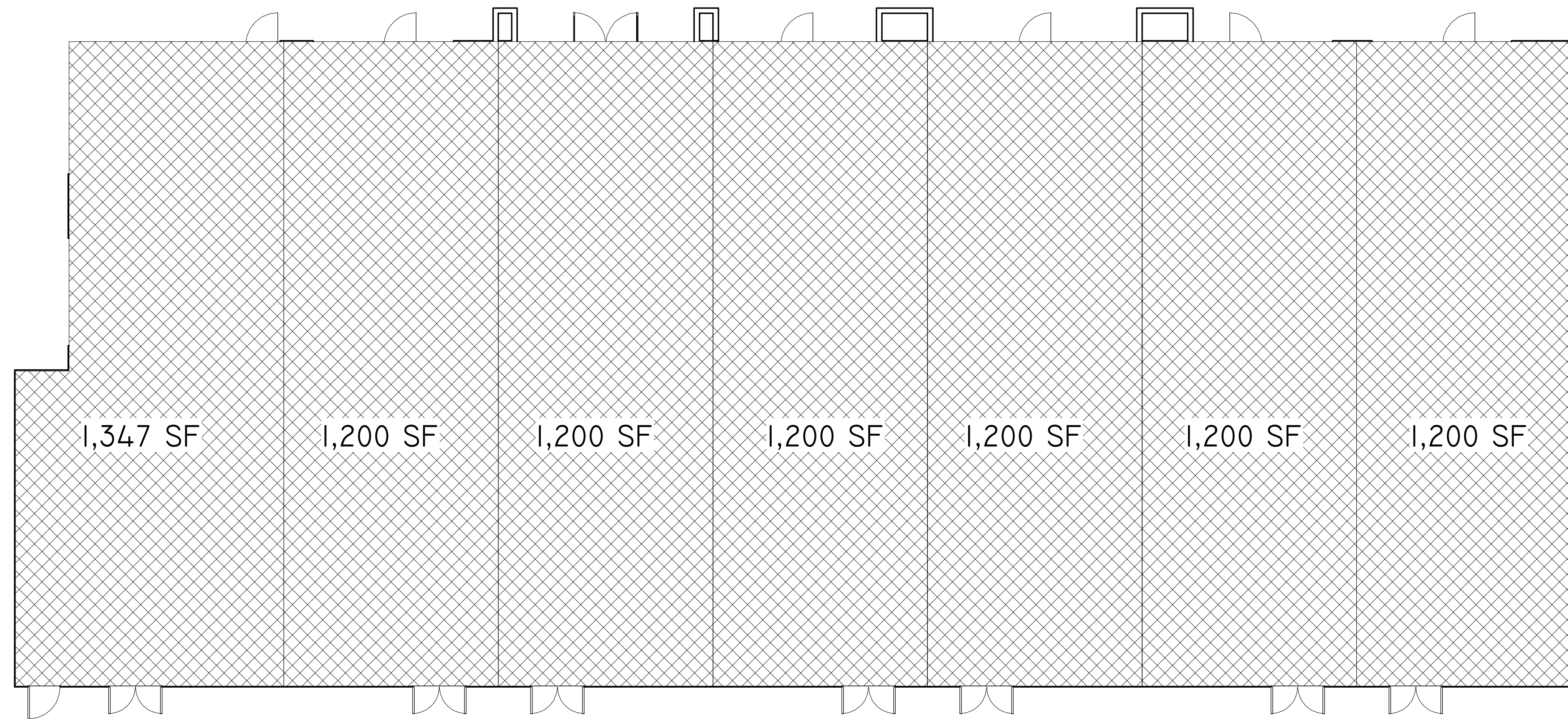
② FLOOR PLAN - BLDG C TENANT SF 1/8" = 1'-0"
