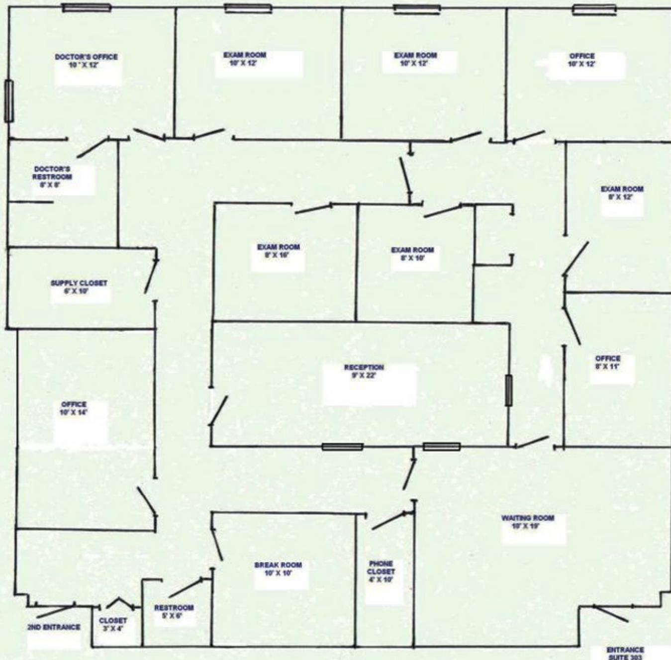
FLOOR PLAN - SUITE 303 111 W. HIGH STREET, ELKTON, MD 21921 2,510 sq. ft.
