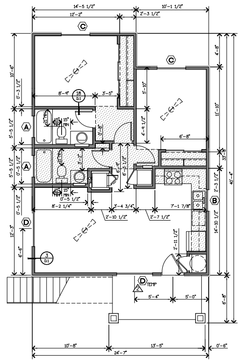
1st FLOOR PLAN SCALE: 1/4"=1'-0"
