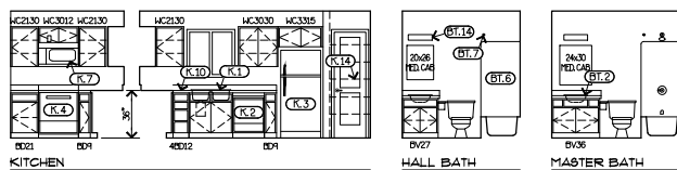
INTERIOR ELEVATIONS SCALE: 1/4"=1'-0"
