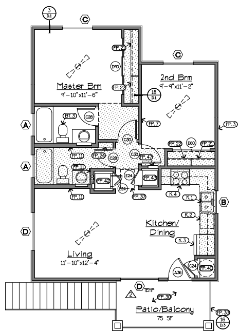
2nd FLOOR PLAN SCALE: 1/4"=1'-0"
