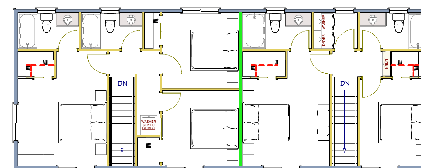
2ND FLOOR LOT # 25 2756 OAKMONT ST. SACRAMENTO CA. 95815 APN #/ 263-0142-025-000
