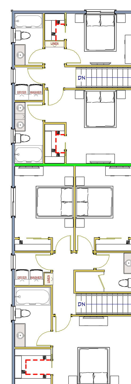
2ND FLOOR LOT # 32 2768 OAKMONT ST. SACRAMENTO CA. 95815 APN #/ 263-0142-032-000
