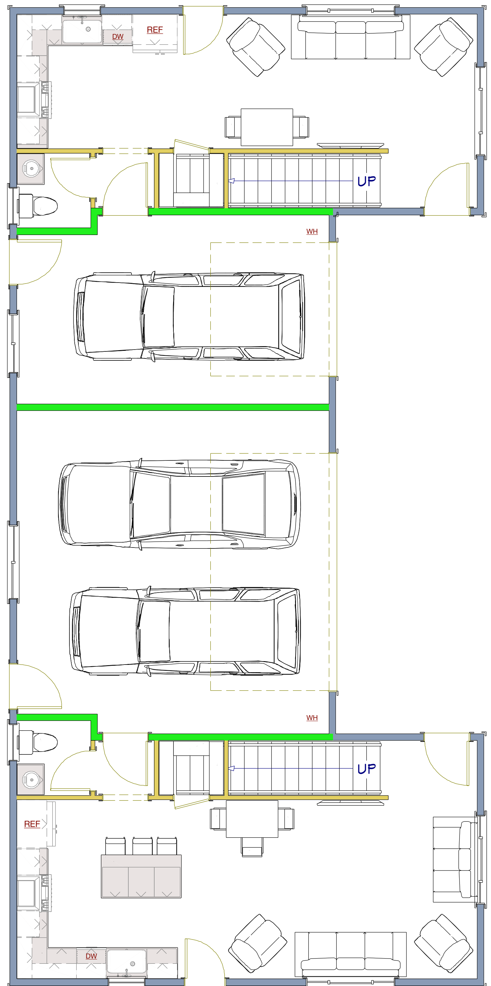
1ST FLOOR LOT # 32 2768 OAKMONT ST. SACRAMENTO CA. 95815 APN #/ 263-0142-032-000
