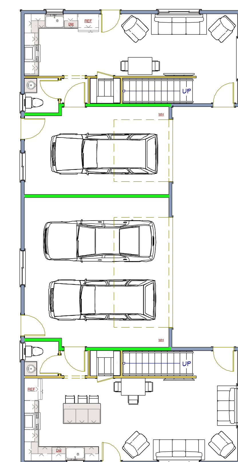
1ST FLOOR LOT # 32 2768 OAKMONT ST. SACRAMENTO CA. 95815 APN #/ 263-0142-032-000
