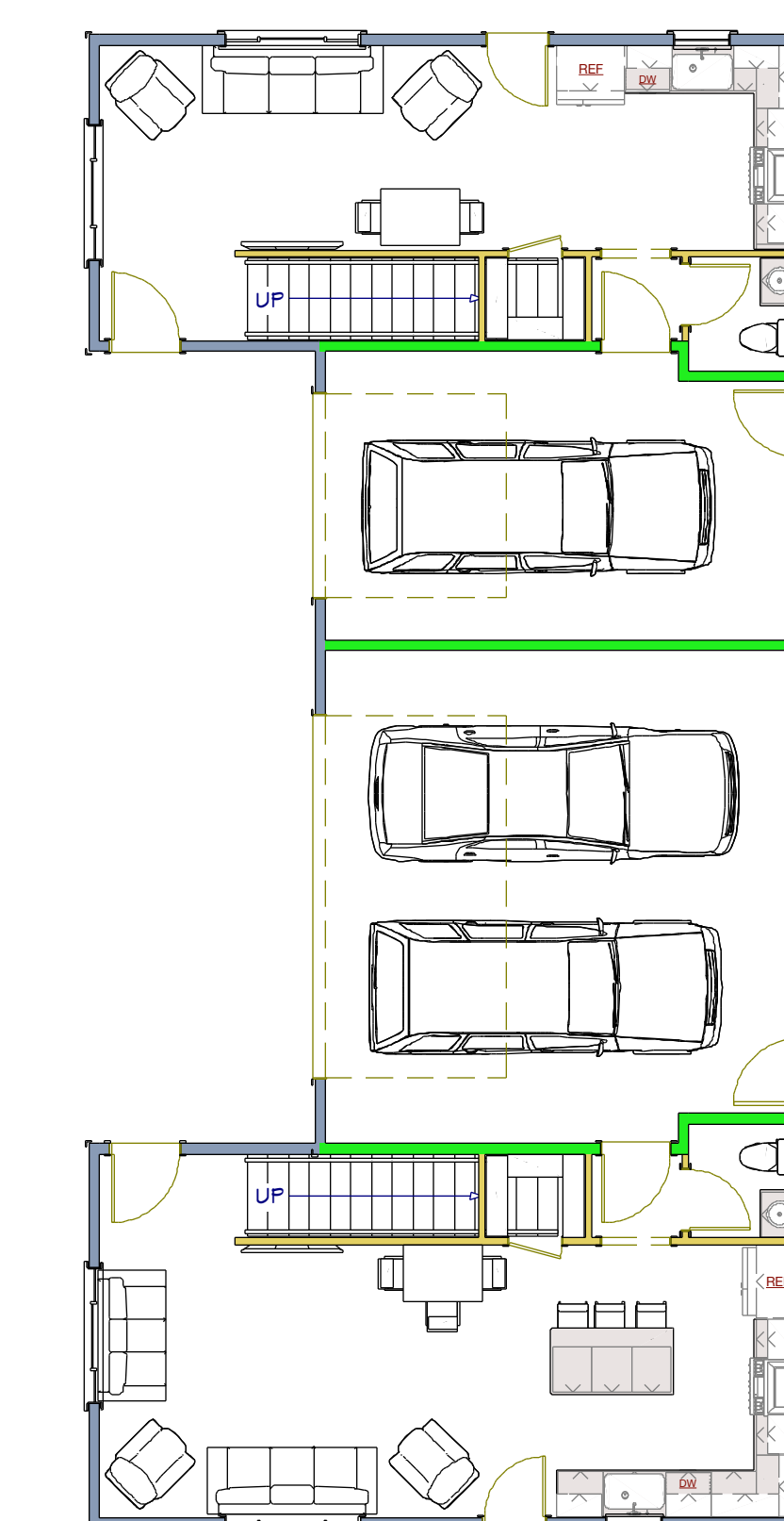
1ST FLOOR LOT # 24 2752 OAKMONT ST. SACRAMENTO CA. 95815 APN #/ 263-0142-024-000
