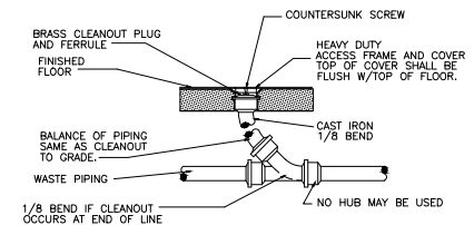
FLOOR CLEANOUT DETAIL NO SCALE
