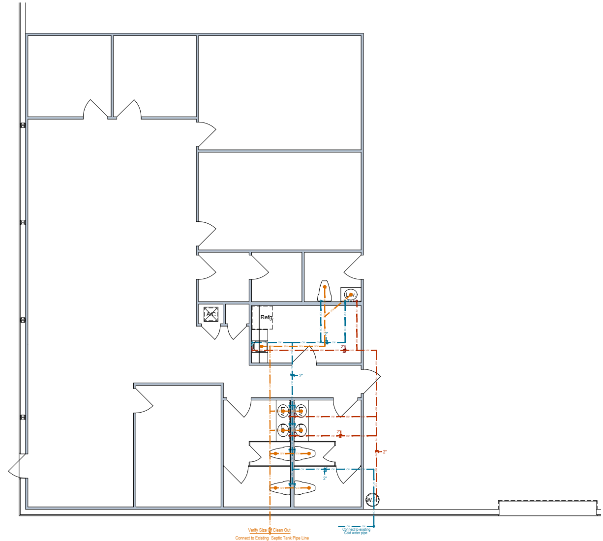
PLUMBING PLAN Scale: 3/16"=1'-0"
