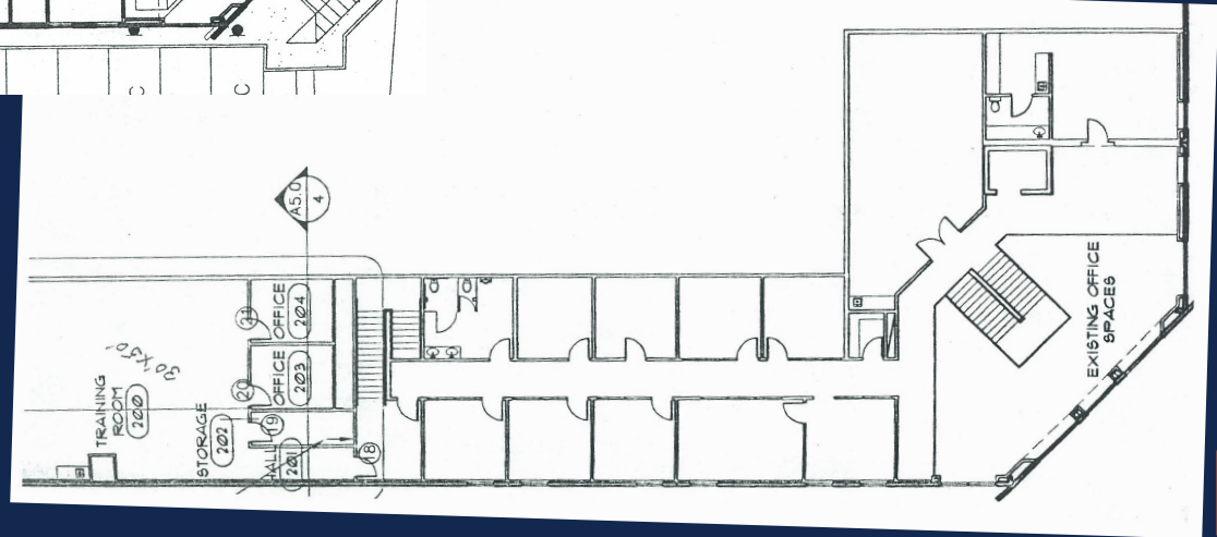
Second Floor
