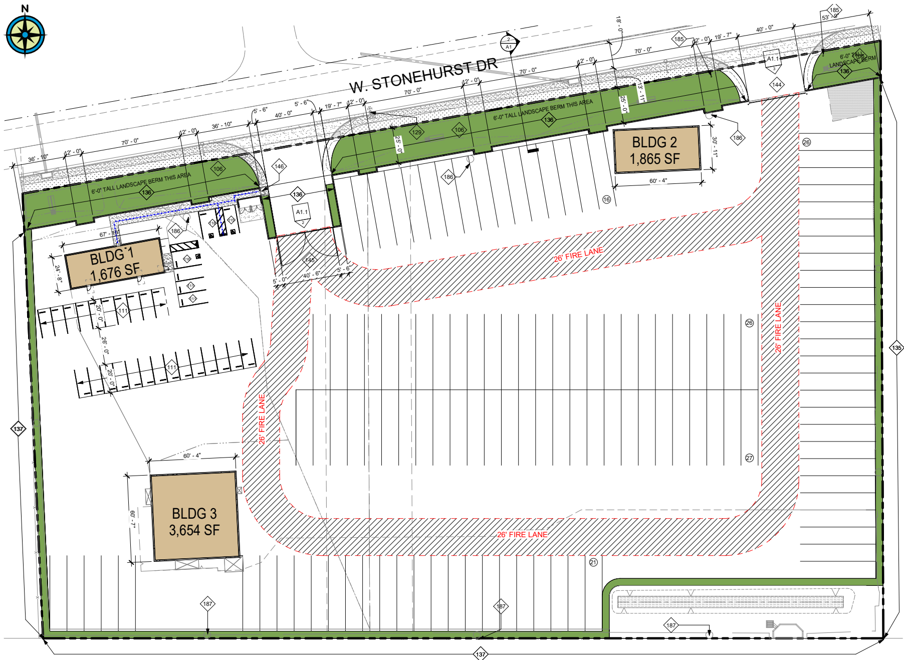
2 PROPOSED SITE PLAN_CD 1" = 30'-0"
