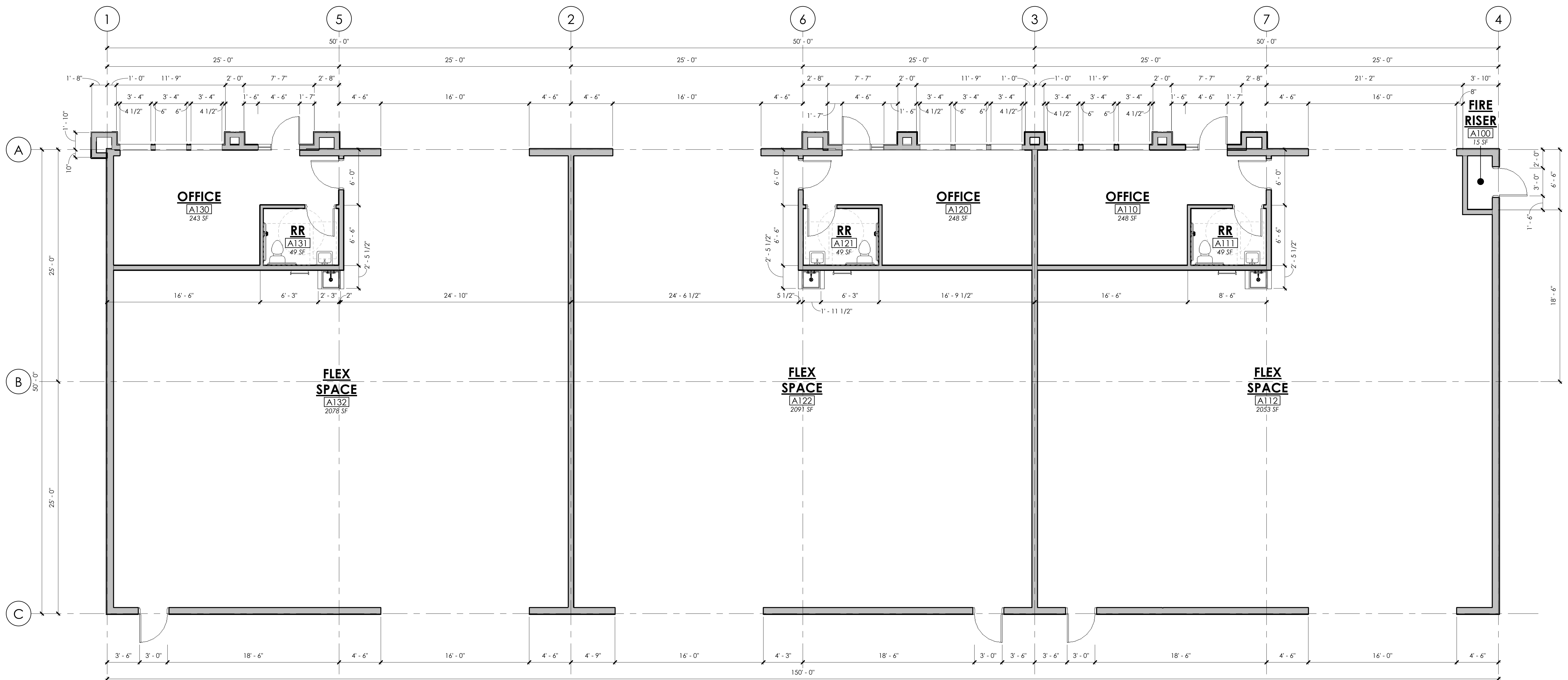
1 FLOOR PLAN 3/16" = 1'-0"
